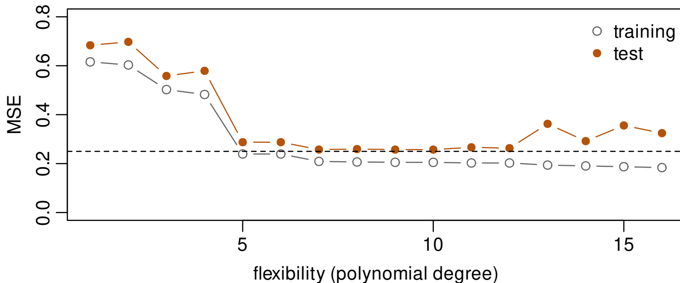
Figure 1.3: Training and test MSE for polynomial fits of increasing degree to 80 observations from y = \sin 2x + x/2 + \varepsilon , \varepsilon \sim N(0, 0.5^2) . The dashed line is \text{var}(\varepsilon) , the irreducible error and the lowest achievable test MSE.
