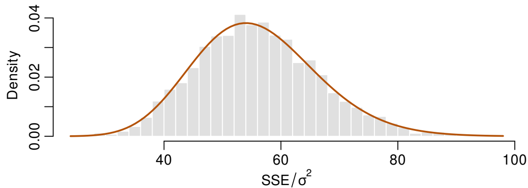
Figure 2.11: Simulated SSE/\sigma^2 over 5000 replications on a fixed design of 60 rows against the \chi_{56}^2 density.
