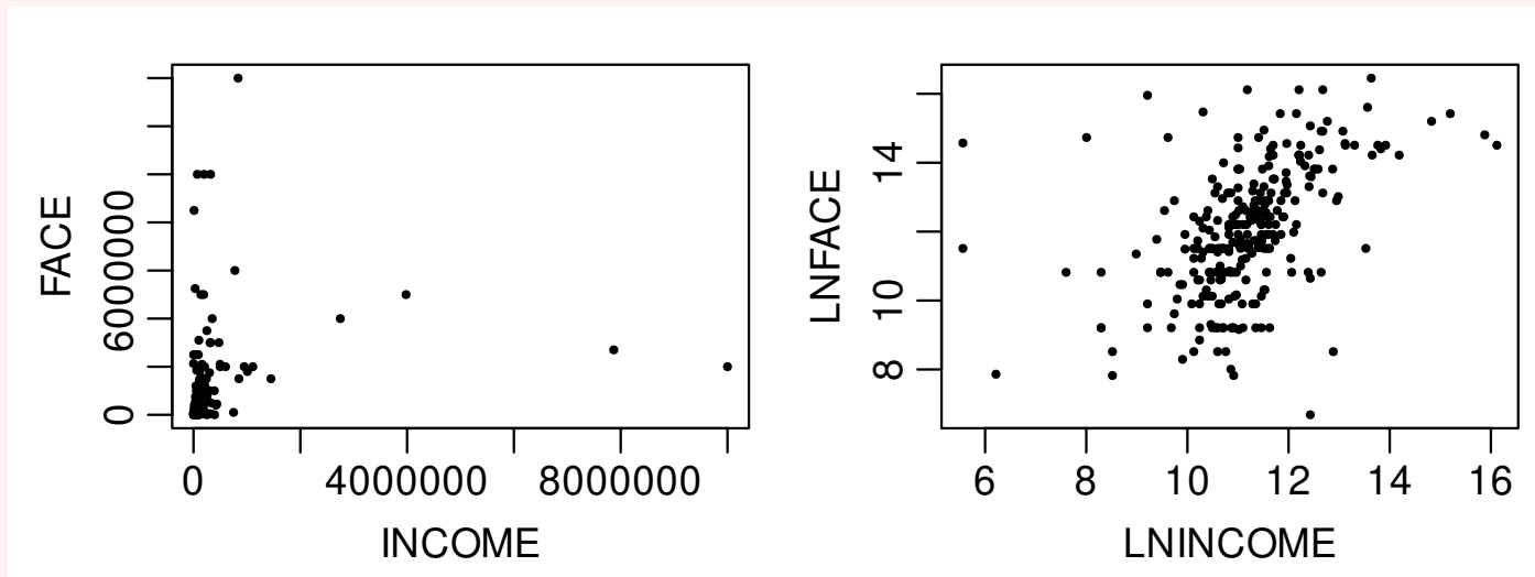
Figure 2.2: Face amount against income, in dollars and in logarithms (FREES Figure 3.1).
