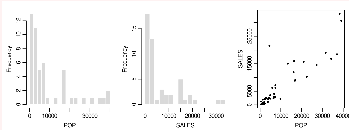
Figure 2.1: The lottery data: histograms of population and of sales, and the scatter plot of sales against population (FREES Figures 2.1–2.2).
