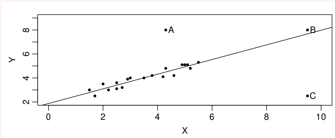
Figure 2.8: Nineteen base points with the line fitted to them, and the three unusual points (FREES Figure 2.7).
