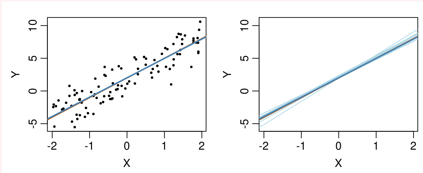
Figure 2.6: Left: the population line 2 + 3X (orange) and the least squares line (blue) for one sample. Right: ten least squares lines from ten samples (ISLR Figure 3.3).
