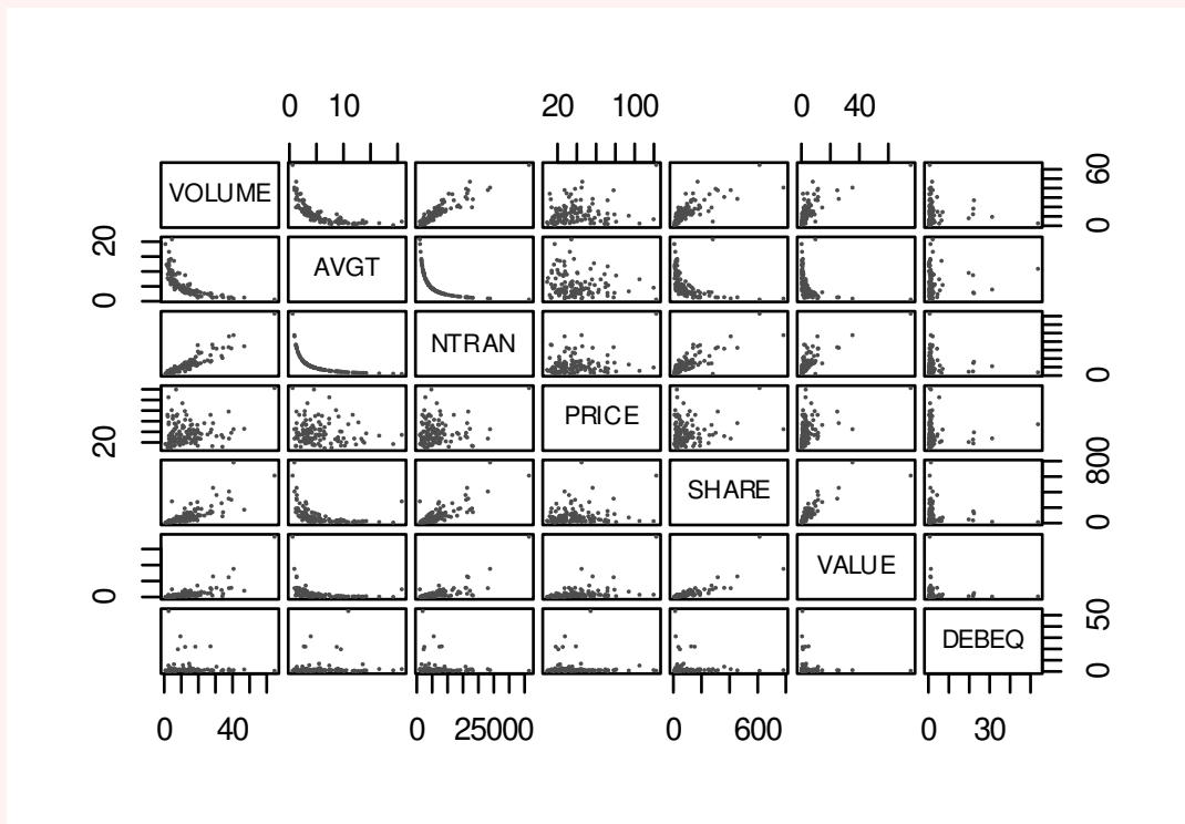
Figure 4.1: The scatterplot matrix of the seven liquidity variables (FREES Figure 5.2): the curved relation of AVGT to NTRAN and the few extreme companies are visible, which the correlation matrix alone does not show.
