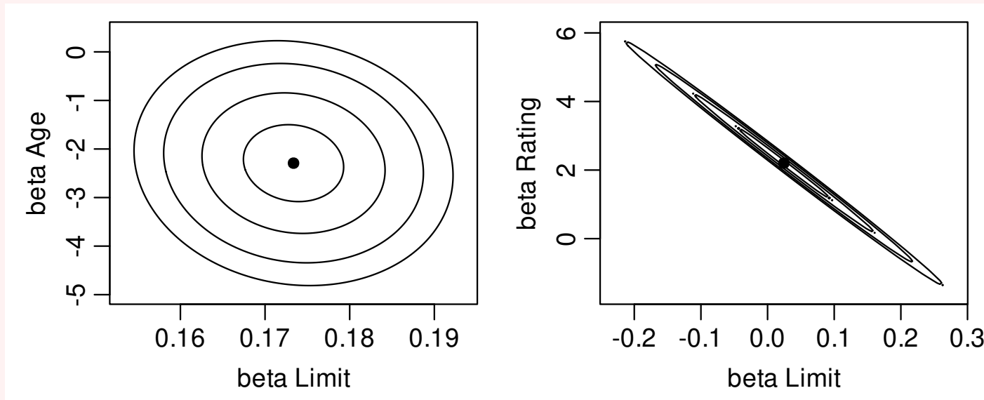
Figure 4.6: Contours of the residual sum of squares, the intercept minimised out, over \pm 4 standard errors of the two slopes, at SSE + 2s^2 F_{2,n-3,1-\alpha} for \alpha = 0.5, 0.1, 0.01, 0.001 (ISLR Figure 3.15).
