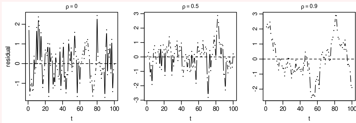
Figure 4.4: Residuals against time for \rho = 0, 0.5 and 0.9 (ISLR Figure 3.10).
