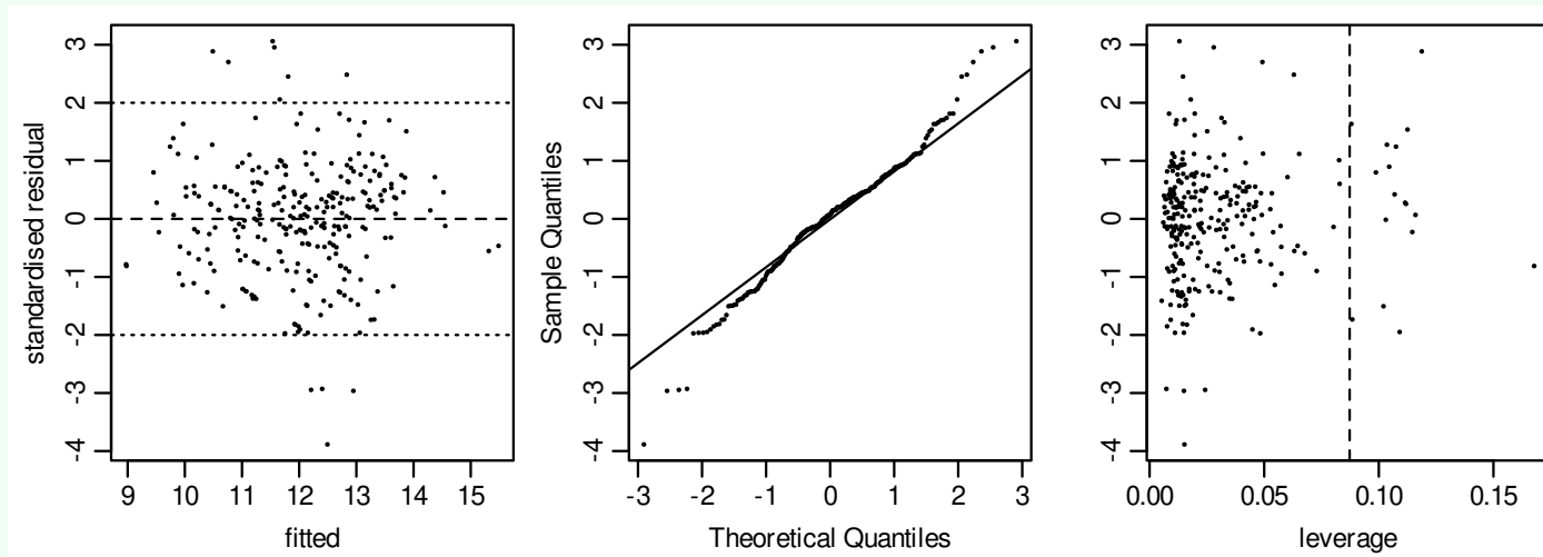
Figure 4.10: Standardised residuals against fitted values, their normal quantile plot, and against leverage, for the regression of LNFACE on seven variables.
