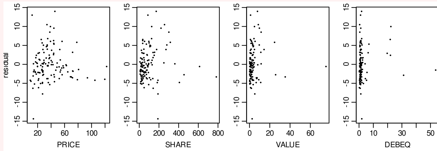
Figure 4.2: Residuals of VOLUME on NTRAN and AVGT against the four remaining candidates (FREES Figure 5.3).
