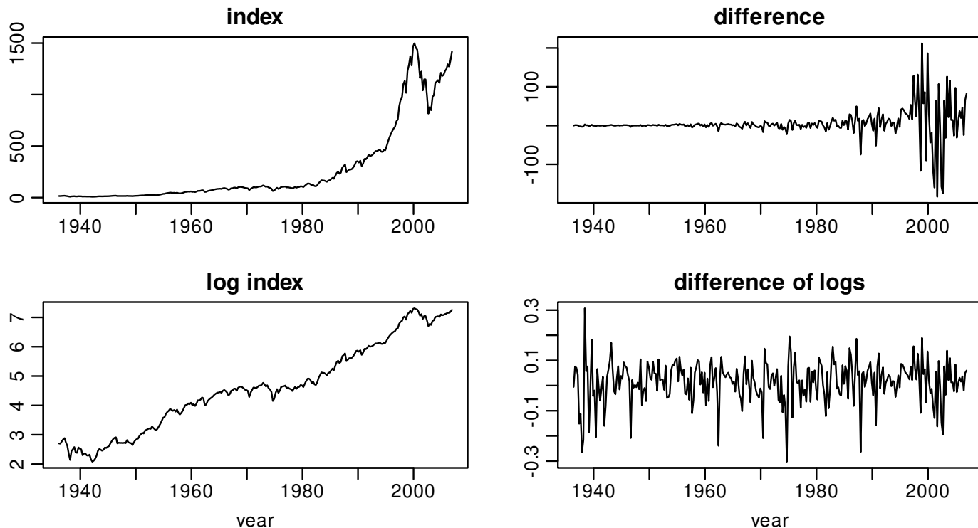
Figure 9.3: The S&P 500 quarterly index, 1936–2006 (FREES Figure 7.9).
