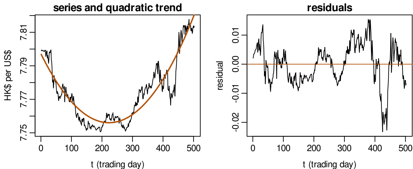
Figure 9.1: Hong Kong exchange rates with the fitted quadratic trend (FREES Figure 7.3), and the residuals, which stay above or below zero for long stretches.
