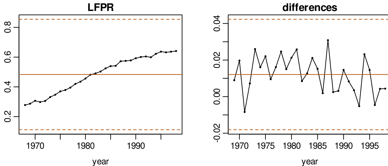
Figure 9.2: Retrospective control charts, with limits \bar{y} \pm 3s_y (dashed), of the labor force participation rates (FREES Figure 7.7) and of their differences.
