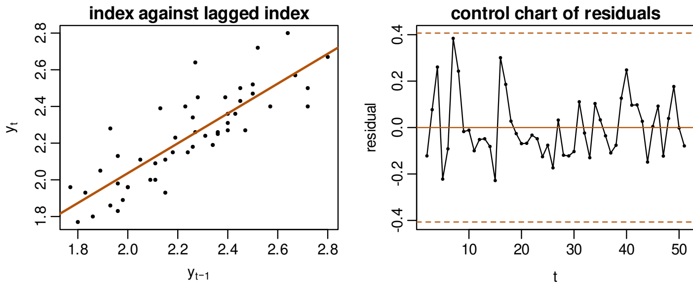
Figure 10.1: Inflation bond index (FREES Figures 8.2 and 8.4): the index against its lagged value with the conditional least squares line, and the control chart of the residuals.
