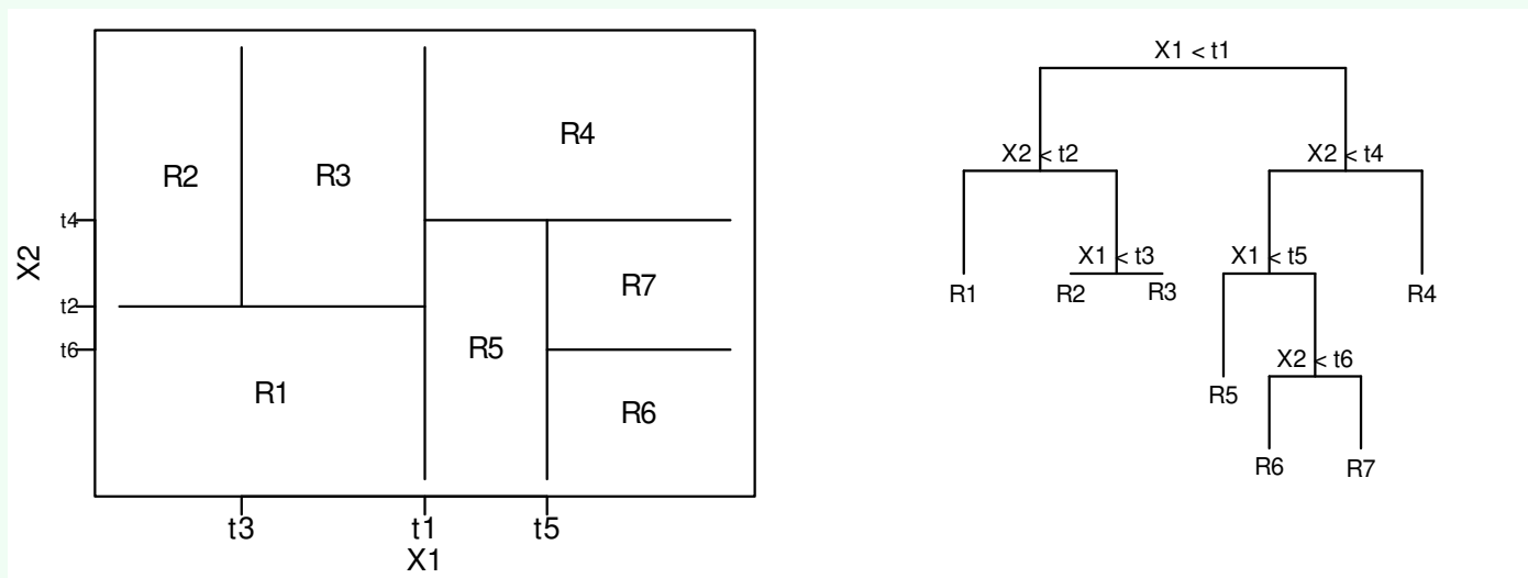
Figure 10.3: A seven-region partition from recursive binary splitting and its tree.
