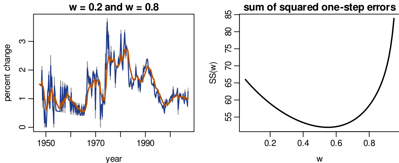
Figure 10.2: Quarterly percentage changes of the medical CPI with exponential smoothing at w = 0.2 and 0.8 (FREES Figure 9.2), and SS(w) (FREES Figure 9.3).
