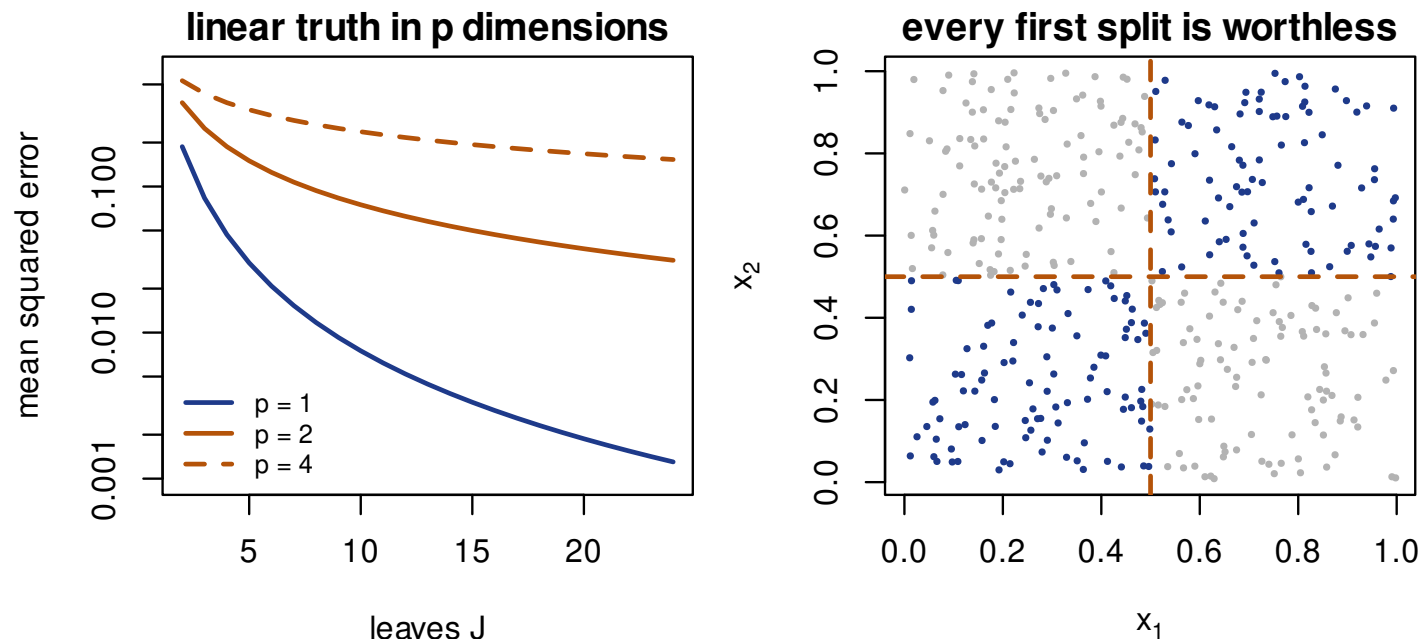
Figure 11.3: Left: Theorem 11.28, the error of the J -box grid approximation to a linear truth, on a log scale; the decay J^{-2/p} flattens as the dimension grows. Right: the checkerboard truth of Theorem 11.30, which four boxes fit exactly and which no single split improves at all.
