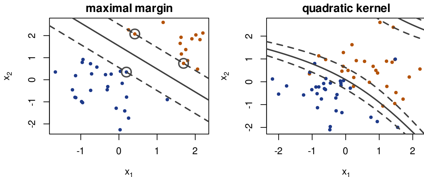
Figure 14.1: Left: the maximal margin hyperplane with its two margin boundaries and the three support vectors circled; by Corollary 14.11 and the remark after it moving any other point, so long as it stays outside the slab on its own side, changes nothing. Right: the same construction with K(\mathbf{x}, \mathbf{z}) = (1 + \mathbf{x}'\mathbf{z})^2 on non-separable data, where the boundary is a conic because the machine is linear in the six features of Example 14.2.
