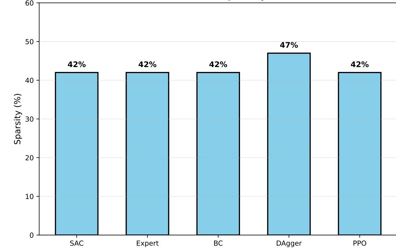
Network Sparsity
