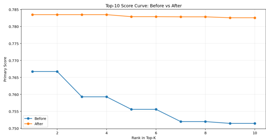
Evidence Figure 2: Top-K Score Curve
