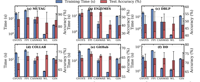
Figure 11: Training time and test accuracy of GRWNN with different RWK evaluators and the WL and GIN baselines.
