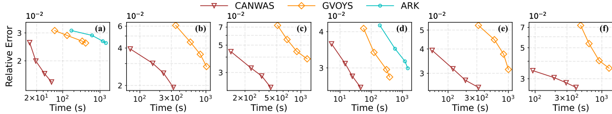
Figure 5: Trade-off between error and running time for single-source RWK query across different algorithms on several graphs: (a) Facebook⊗Facebook, (b) Facebook⊗Youtube, (c) Facebook⊗Orkut, (d) GrQc⊗GrQc, (e) GrQc⊗Youtube, and (f) GrQc⊗Orkut.
