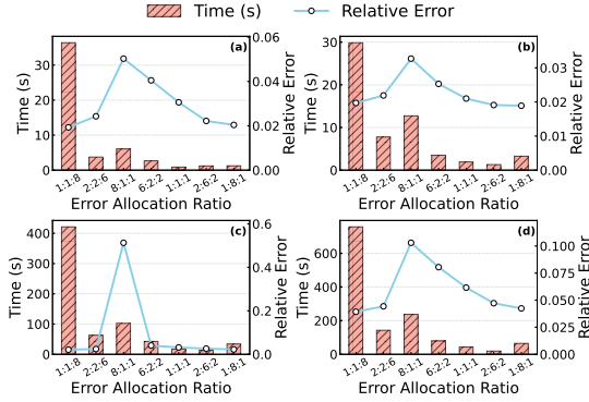
Figure 7: Effect of error budget allocation on two representative graphs: (a) (b) MUTAG and (c) (d) Facebook \otimes Facebook. The x-axis labels denote the allocation ratio \epsilon_t : \epsilon_r : \epsilon_w .
