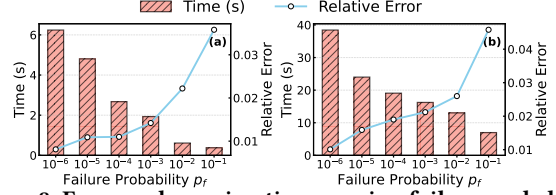
Figure 8: Error and running time varying failure probability on two networks: (a) MUTAG and (b) Facebook \otimes Facebook.
