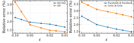
Figure 6: Mean relative error versus \epsilon .
