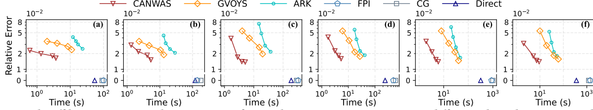
Figure 3: Trade-off between error and running time for single-source RWK query across different algorithms on several graphs: (a) MUTAG, (b) ENZYMES, (c) DBLP, (d) COLLAB, (e) Github, and (f) DD.
