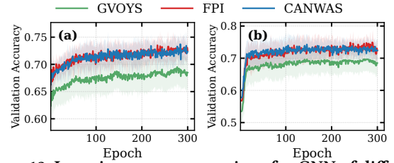
Figure 12: Learning curve comparison for GNN of different methods: (a) COLLAB and (b) DD.
