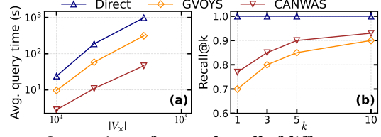
Figure 10: Comparison of cost and recall of different methods.
