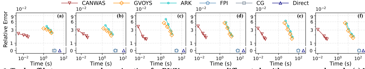
Figure 2: Trade-off between error and running time for RWK query across different algorithms on several graphs: (a) MUTAG, (b) ENZYMES, (c) DBLP, (d) COLLAB, (e) Github, and (f) DD.
