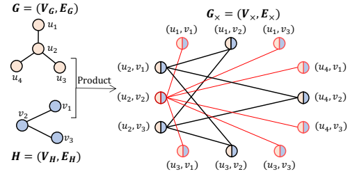
Figure 1: Toy example of a product graph.
