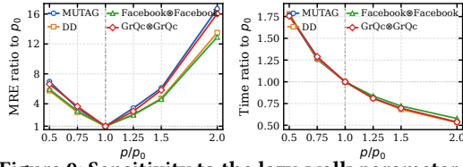
Figure 9: Sensitivity to the lazy-walk parameter p .
