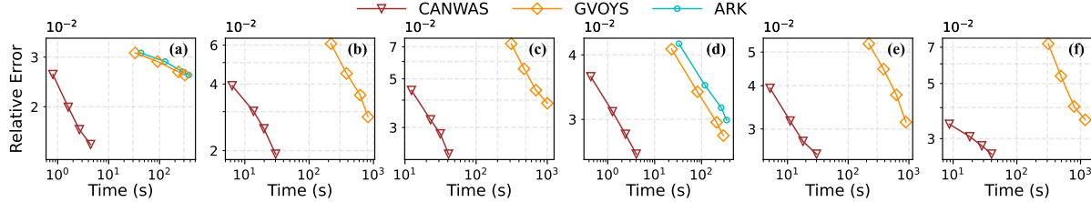
Figure 4: Trade-off between error and running time for RWK query across different algorithms on several graphs: (a) Facebook⊗Facebook, (b) Facebook⊗Youtube, (c) Facebook⊗Orkut, (d) GrQc⊗GrQc, (e) GrQc⊗Youtube, and (f) GrQc⊗Orkut.
