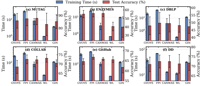
Figure 11: Training time and test accuracy of GRWNN with different RWK evaluators and the WL and GIN baselines.
