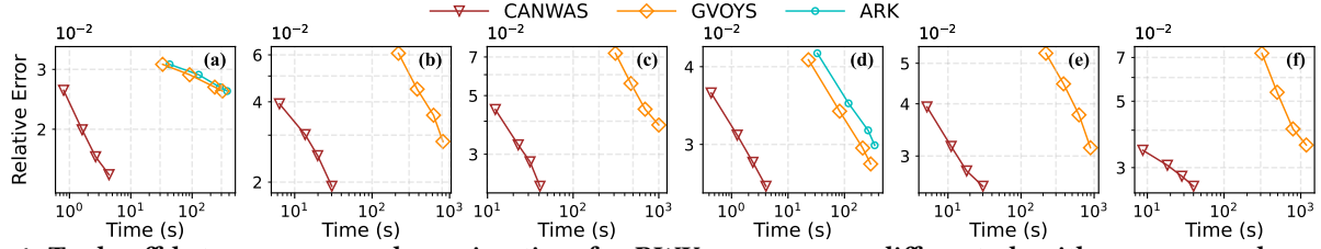
Figure 4: Trade-off between error and running time for RWK query across different algorithms on several graphs: (a) Facebook⊗Facebook, (b) Facebook⊗Youtube, (c) Facebook⊗Orkut, (d) GrQc⊗GrQc, (e) GrQc⊗Youtube, and (f) GrQc⊗Orkut.
