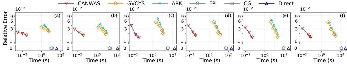
Figure 2: Trade-off between error and running time for RWK query across different algorithms on several graphs: (a) MUTAG, (b) ENZYMES, (c) DBLP, (d) COLLAB, (e) Github, and (f) DD.
