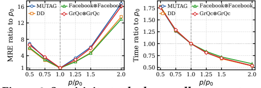
Figure 9: Sensitivity to the lazy-walk parameter p .
