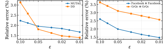
Figure 6: Mean relative error versus \epsilon .
