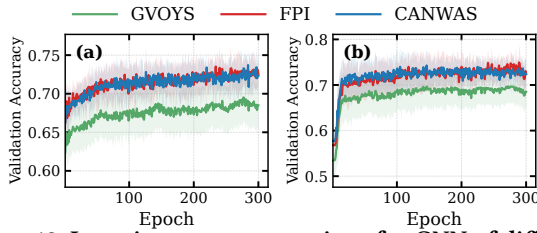
Figure 12: Learning curve comparison for GNN of different methods: (a) COLLAB and (b) DD.
