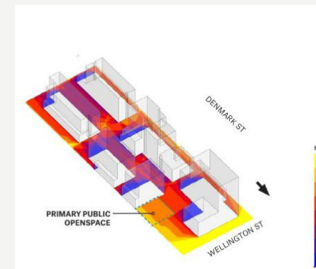
SOLAR ANALYSIS / GRASSHOPPER + LADYBUG
