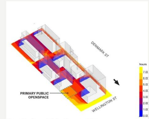
SOLAR ANALYSIS / GRASSHOPPER + LADYBUG
