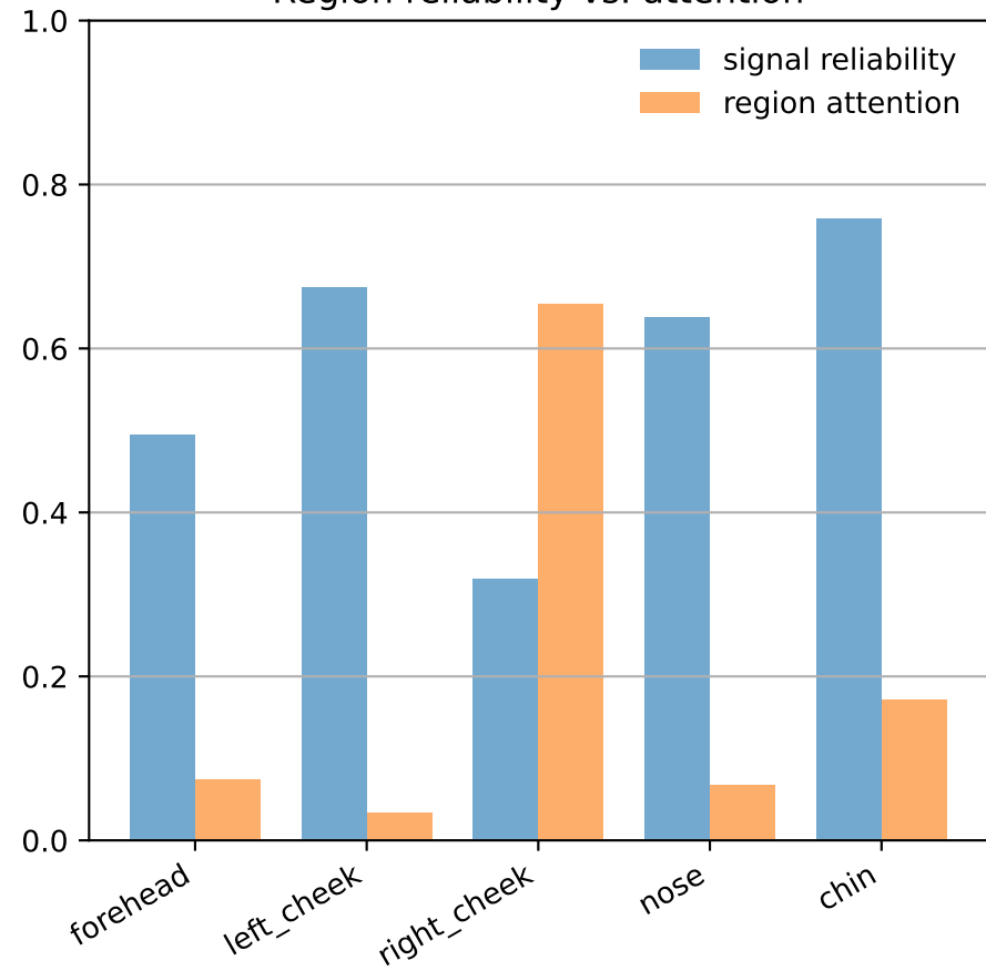
Region reliability vs. attention
