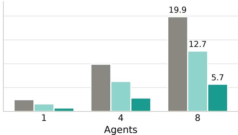
16,321-Token Prefix
