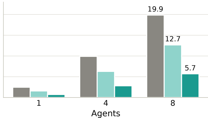
16,321-Token Prefix
