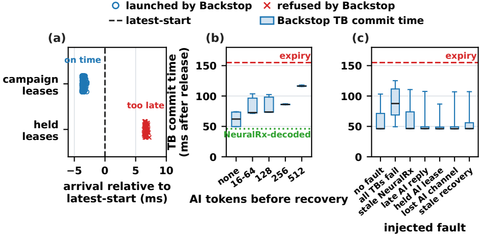
Fig. 15. Execution refinement and radio commit time. (a) Arrival of each AI lease at the Qwen worker relative to its absolute latest-start: the 1,077 leases of the two-node campaign and the 52 leases that the held-lease fault keeps past the latest-start. (b) Commit time of every recovered TB in the two-node campaign, grouped by the prompt length of the AI lease that runs before its recovery; the dotted line marks the median commit of the TBs that NeuralRx decodes. (c) Commit time of every TB under each injected fault: no fault, all TBs of a period fail, stale and duplicate NeuralRx outcomes, a late AI reply after GPU completion, an AI lease held past its latest-start, an AI channel lost before GPU completion, and stale and duplicate recovery responses.
