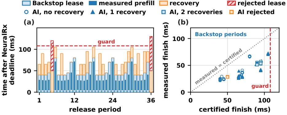
Fig. 12. Online scheduling in the two-node campaign, measured from the NeuralRx deadline. (a) Certificate of the shared lane in 36 consecutive release periods: each admitted AI lease includes the 5 ms launch-control charge, and the required recoveries follow it with their full bound; a rejected AI lease is drawn where it would end. (b) Measured against certified finish of the last action on the shared lane, the AI prefill or the last recovery, in all 1,200 periods; the marker gives the required recoveries of the period, orange marks a rejected AI unit, and the dotted diagonal marks equality.
