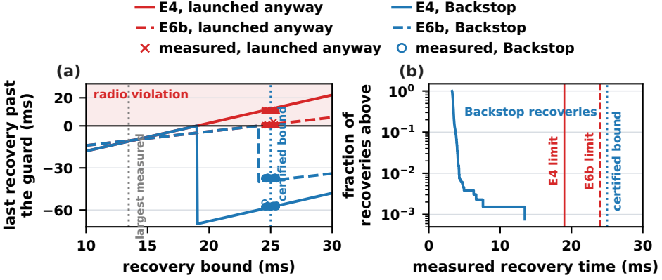
Fig. 17. Sensitivity to the recovery bound. (a) End of the last recovery relative to the guard when the unit that Backstop rejects runs anyway, against the recovery bound B_{\text{conv}} : lines follow the bound-respecting schedules of E4 and E6b, and crosses mark the physical attempts measured at the certified 25 ms bound. (b) Fraction of the 1,312 measured recovery times of the two-node campaign that exceed a given length, with the bounds at which E4 and E6b disappear (E4 and E6b limits) and the certified bound.
