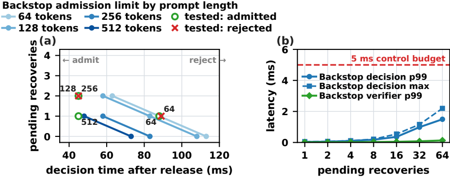
Fig. 16. Predictive scheduling and control cost. (a) Latest decision time at which one AI unit of each prompt length remains admissible with four admitted TBs and zero to four pending recoveries; circles and crosses mark the prespecified physical tests that the scheduler admitted and rejected, labeled with their prompt length. (b) Candidate construction and independent verification latency against the number of pending recoveries, with the evaluated 5 ms control budget. Latencies are finite-run measurements, not WCETs.
