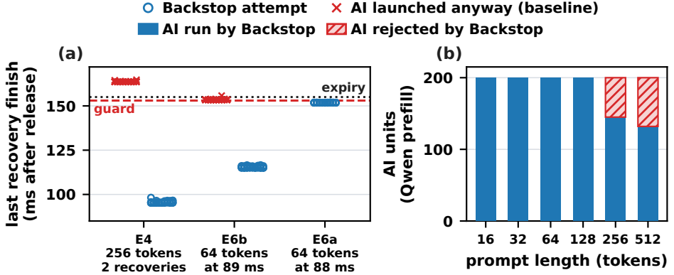
Fig. 14. Radio safety at the certificate boundary on two nodes. (a) End of the last recovery in every attempt of the bound-padded boundary diagnostic. E4 offers a 256-token unit with two required recoveries at 45 ms; E6b and E6a offer a 64-token unit with one required recovery at 89 and 88 ms. Baseline attempts launch the unit anyway: idle-time admission in E4 and a shadow launch of the unit that Backstop rejects in E6b. (b) AI units per prompt length in the two-node campaign: units that Backstop runs and units that it rejects because they break the certified recovery bound; idle-time admission would run all of them, and static reservation runs none.
