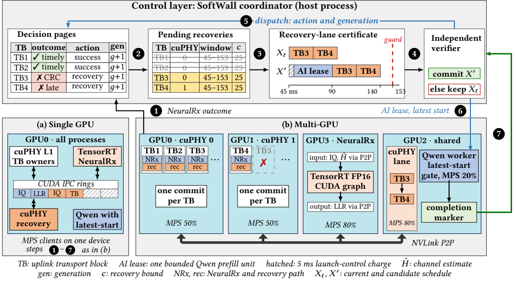
Fig. 5. SoftWall architecture for one release period. Steps: NeuralRx outcome (①), outcome batch (②), recovery retiming (③), independent verification (④), dispatch (⑤), AI lease (⑥), and completion marker (⑦). The steps are drawn for the evaluated multi-GPU placement (b); the single-GPU placement (a) exchanges IQ, LLR, and TB buffers through CUDA IPC rings and uses the same steps. In (b), cuPHY instance 0 owns TB1-TB3, instance 1 owns TB4 and TB5, and ellipses mark further TBs.
