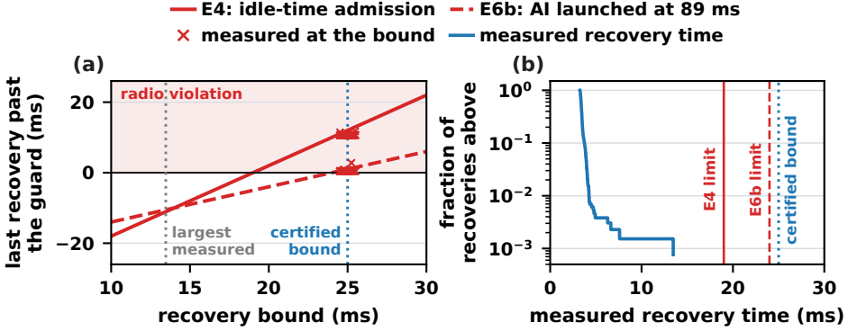
Fig. 16. Sensitivity to the recovery bound. (a) End of the last recovery relative to the guard when the unit that SoftWall rejects runs anyway, against the recovery bound B_{\text{conv}} : lines follow the bound-respecting schedules of E4 and E6b, and crosses mark the physical attempts measured at the certified 25 ms bound. (b) Fraction of the 1,312 measured recovery times of the two-node campaign that exceed a given length, with the bounds at which E4 and E6b disappear (E4 and E6b limits) and the certified bound.
