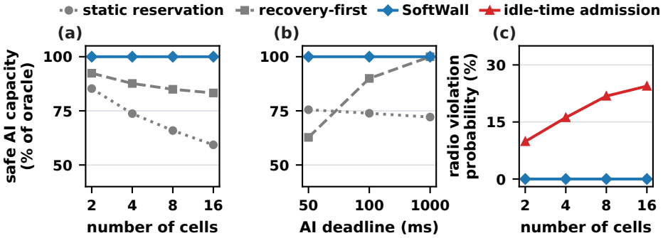
Fig. 9. Safe AI capacity in the exact-checked capacity model (13,716 mandatory-feasible points). (a) AI capacity relative to the offline oracle as the number of cells grows. (b) AI capacity as the AI deadline tightens. (c) Radio violation probability of idle-time admission; static reservation, recovery-first, and SoftWall never violate the all-fail schedule. Idle-time admission is omitted from (a) and (b) because the AI that it admits exceeds the safe capacity.
