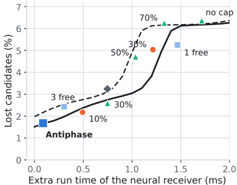
(a) Candidates that find no free neural receiver
