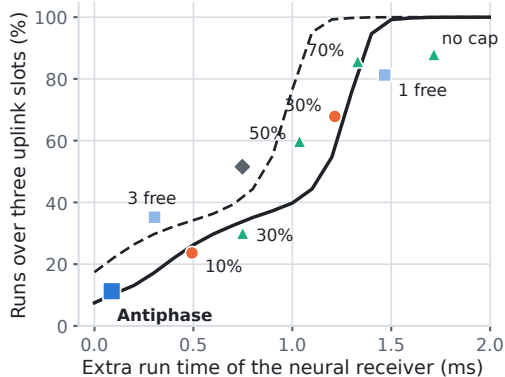
(b) Neural receiver runs over three slots
