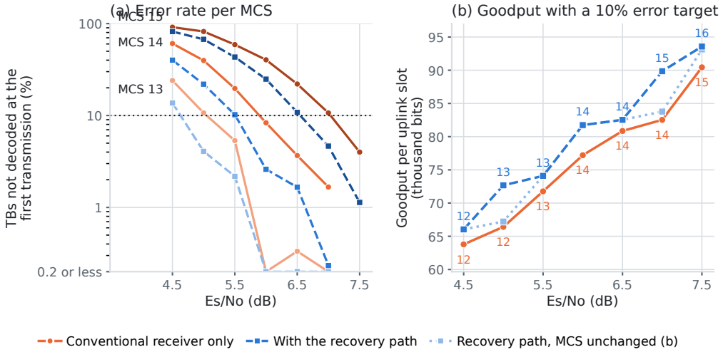
Fig. 10. Link adaptation with the recovery path (two-user cell, low-correlation channel, 300 TBs per point). Dotted line in (a): 10% target. Numbers in (b): MCS chosen.
