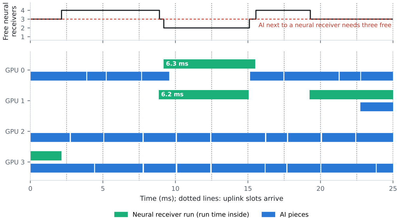
Backstop: measured run, uplink slots 3232-3241
