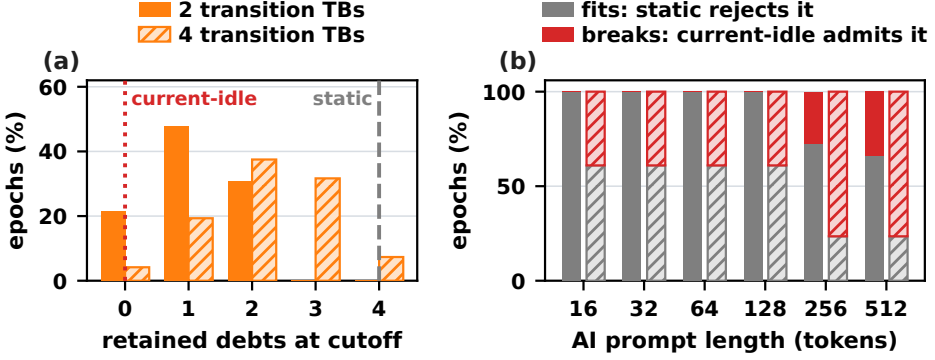
Fig. 2. Measured recovery debt in the evaluated warm mode (1,200 epochs on two nodes). (a) Retained debts at the 45 ms common cutoff for epochs with two transition-SNR TBs, and for 600 four-TB epochs that join the transition TBs of consecutive measured epochs. The dotted line marks the zero debt that current-idle admission sees; the dashed line marks the four recoveries that static reservation holds. (b) All-fail certificate decision per AI prompt length. A unit either fits, and static reservation rejects it, or breaks the all-fail recovery bound, and current-idle admission accepts it. Solid bars are the measured decisions; hatched bars apply the same rule, which reproduces all 1,200 measured decisions, to the joined four-TB epochs.
