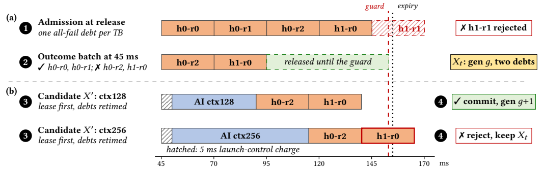
Fig. 4. One transaction on the shared lane. (a) Admission reserves one all-fail recovery per TB and rejects h1-r1; the 45 ms batch deletes two debts in one generation. (b) The verifier commits the context-128 lease and keeps X_t for the context-256 lease, whose last recovery would end after the guard.
