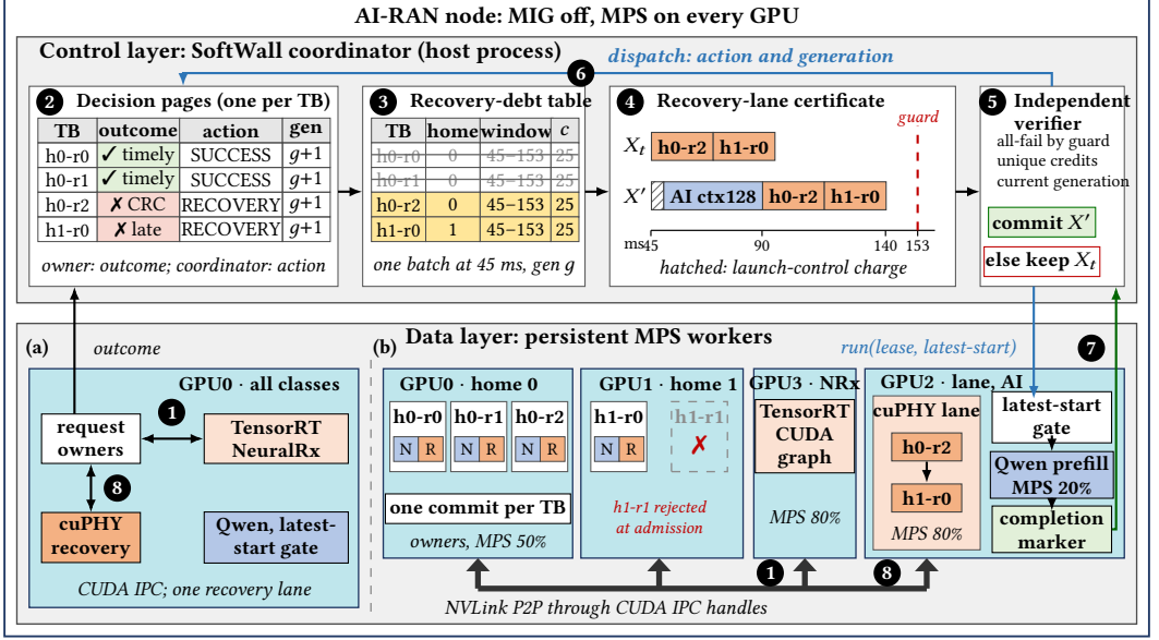
Fig. 3. SoftWall architecture. The control layer is identical for every placement: steps (2)–(7) record outcomes, apply one cutoff batch, retime debts around a candidate lease, verify it, dispatch actions and the lease, and retire the lease on a marker. The data layer shows (a) one GPU over CUDA IPC and (b) the evaluated four-GPU placement over NVLink P2P, with NeuralRx input (1) and certificate-ordered recovery (8).
