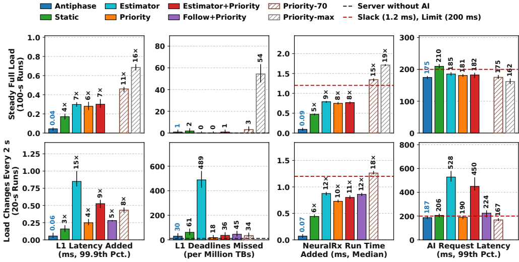
Fig. 12. What AI adds to the latency of the radio work, and the latency of the AI requests (16 cells, four GPUs, five seeds; lines: range over seeds, for the misses the 95% interval). Top: runs of 100 s without their first 20 s. Bottom: runs of 20 s without their first 5 s. L1 latency: samples arrive until the conventional result. The number on a baseline is how many times more it adds than Antiphase.
