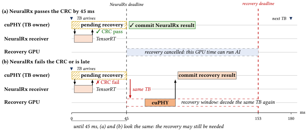
Fig. 1. One uplink TB in one 180 ms period of our test timeline, which is slower than 5G slot timing. cuPHY receives the TB and hands it to NeuralRx at once, and until the 45 ms NeuralRx deadline the TB has a pending recovery that no GPU queue contains. (a) If the NeuralRx result passes the CRC, cuPHY commits it, and the recovery is cancelled. (b) If the result fails the CRC, is late, or is missing, cuPHY decodes the same TB again on the recovery GPU before the 153 ms recovery deadline.
