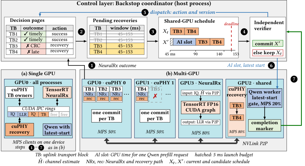
Fig. 5. Backstop architecture for one period. Steps: NeuralRx result (①), all results applied at the NeuralRx deadline (②), recoveries rescheduled around an AI slot (③), independent check (④), actions sent (⑤), AI slot sent (⑥), and completion marker (⑦). The steps are drawn for the evaluated four-GPU node (b); on one GPU (a), the same processes exchange IQ, LLR, and TB buffers through CUDA IPC rings and follow the same steps. Each TB comes from a different cell; cuPHY instance 0 owns TB1-TB3, instance 1 owns TB4 and TB5, and ellipses mark further TBs.
