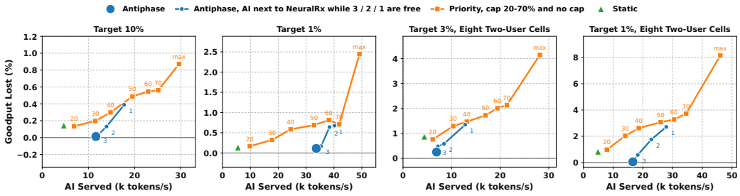
Fig. 12. AI served against the goodput of the two-user cells that is lost, with the outer loop (two seeds; all policies of a panel run in one job). Orange: low-priority AI with a cap of 20-70% and without a cap. Blue: Antiphase, and its settings that allow AI next to a neural receiver while 3, 2, or 1 neural receivers are free.
