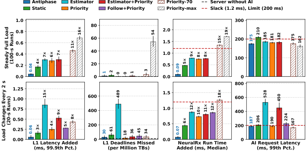
Fig. 13. What AI adds to the latency of the radio work, and the latency of the AI requests (16 cells, four GPUs, five seeds; lines: range over seeds, for the misses the 95% interval). Top: runs of 100 s without their first 20 s. Bottom: runs of 20 s without their first 5 s. L1 latency: samples arrive until the conventional result. The number on a baseline is how many times more it adds than Antiphase.
