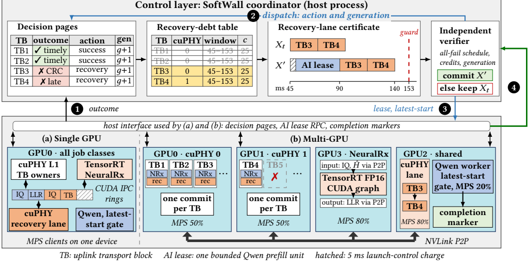
Fig. 3. SoftWall architecture. Both placements reach the coordinator through one host interface. (1) Each owner publishes its NeuralRx outcome to a decision page. One common-cutoff batch then updates the debt table, the scheduler retimes retained debts around a candidate lease, and the independent verifier commits X' or keeps X_t . (2) The coordinator publishes each action with its generation and (3) sends the lease with an absolute latest-start through the AI lease RPC. (4) A completion or non-launch marker retires the lease. The shared lane runs retained recoveries in certificate order. In (a), the processes on one GPU exchange IQ, LLR, and TB buffers through CUDA IPC rings. In (b), the evaluated multi-GPU placement uses NVLink P2P; cuPHY instance 0 owns TB1–TB3, instance 1 owns TB4 and TB5, and ellipses mark further TBs.
