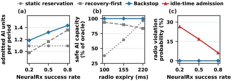
Fig. 10. Drivers of safe AI capacity in the exact-checked capacity model. (a) Mean AI units per release period against the NeuralRx success rate. (b) AI capacity relative to the offline oracle against the radio expiry. (c) Radio violation probability of idle-time admission against the NeuralRx success rate. Each success rate covers the same 4,572 mandatory-feasible configurations.
