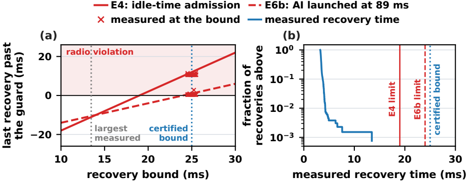
Fig. 16. Sensitivity to the recovery bound. (a) End of the last recovery relative to the guard when the unit that Backstop rejects runs anyway, against the recovery bound B_{\text{conv}} : lines follow the bound-respecting schedules of E4 and E6b, and crosses mark the physical attempts measured at the certified 25 ms bound. (b) Fraction of the 1,312 measured recovery times of the two-node campaign that exceed a given length, with the bounds at which E4 and E6b disappear (E4 and E6b limits) and the certified bound.
