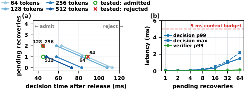
Fig. 15. Predictive scheduling and control cost. (a) Latest decision time at which one AI unit of each prompt length remains admissible with four admitted TBs and zero to four pending recoveries; circles and crosses mark the prespecified physical tests that the scheduler admitted and rejected, labeled with their prompt length. (b) Candidate construction and independent verification latency against the number of pending recoveries, with the evaluated 5 ms control budget. Latencies are finite-run measurements, not WCETs.
