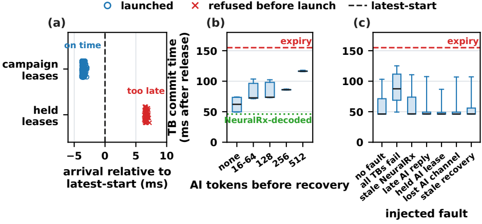
Fig. 14. Execution refinement and radio commit time. (a) Arrival of each AI lease at the Qwen worker relative to its absolute latest-start: the 1,077 leases of the two-node campaign and the 52 leases that the held-lease fault keeps past the latest-start. (b) Commit time of every recovered TB in the two-node campaign, grouped by the prompt length of the AI lease that runs before its recovery; the dotted line marks the median commit of the TBs that NeuralRx decodes. (c) Commit time of every TB under each injected fault: no fault, all TBs of a period fail, stale and duplicate NeuralRx outcomes, a late AI reply after GPU completion, an AI lease held past its latest-start, an AI channel lost before GPU completion, and stale and duplicate recovery responses.
