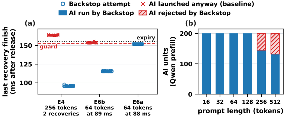
Fig. 13. Radio safety at the certificate boundary on two nodes. (a) End of the last recovery in every attempt of the bound-padded boundary diagnostic. E4 offers a 256-token unit with two required recoveries at 45 ms; E6b and E6a offer a 64-token unit with one required recovery at 89 and 88 ms. Baseline attempts launch the unit anyway: idle-time admission in E4 and a shadow launch of the unit that Backstop rejects in E6b. (b) AI units per prompt length in the two-node campaign: units that Backstop runs and units that it rejects because they break the certified recovery bound; idle-time admission would run all of them, and static reservation runs none.
