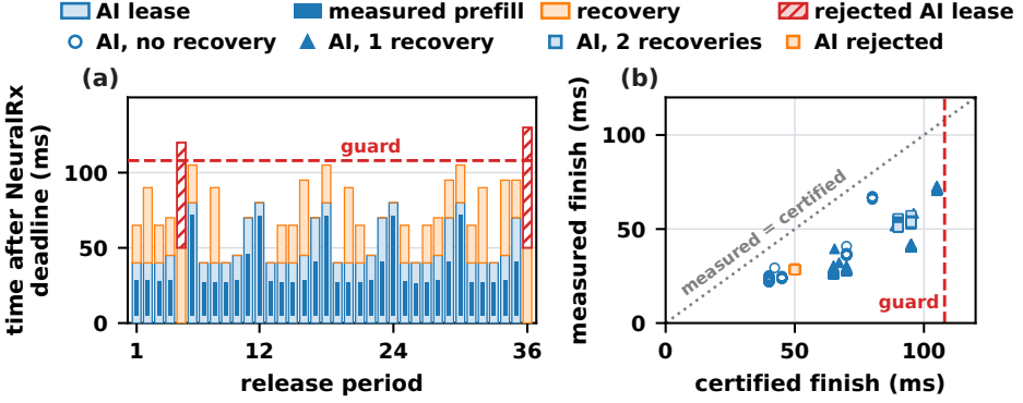
Fig. 12. Online scheduling in the two-node campaign, measured from the NeuralRx deadline. (a) Certificate of the shared lane in 36 consecutive release periods: each admitted AI lease includes the 5 ms launch-control charge, and the required recoveries follow it with their full bound; a rejected AI lease is drawn where it would end. (b) Measured against certified finish of the last action on the shared lane, the AI prefill or the last recovery, in all 1,200 periods; the marker gives the required recoveries of the period, orange marks a rejected AI unit, and the dotted diagonal marks equality.
