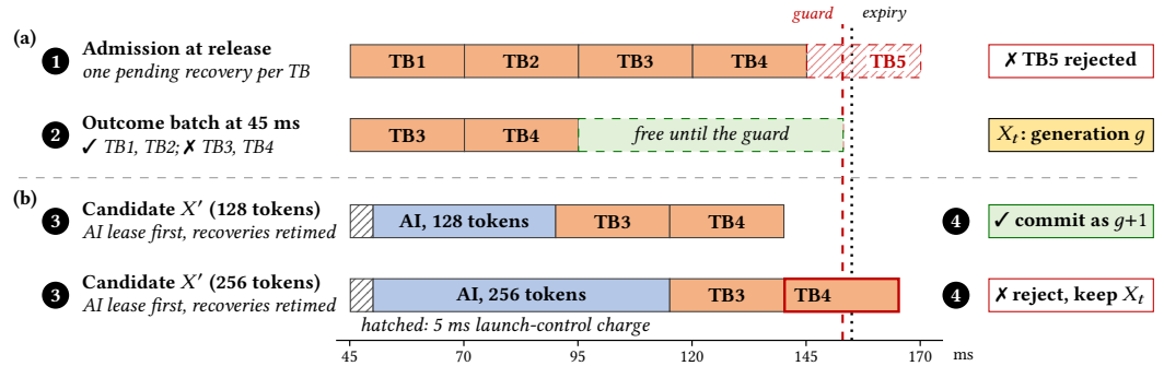
Fig. 6. One transaction on the shared lane. (a) Admission reserves one all-fail recovery per TB and rejects TB5; the 45 ms batch cancels two pending recoveries in one generation. (b) The verifier commits the 128-token AI lease and keeps X_t for the 256-token AI lease, whose last recovery would end after the guard. AI units are Qwen prefill requests; hatching marks the 5 ms launch-control charge.
