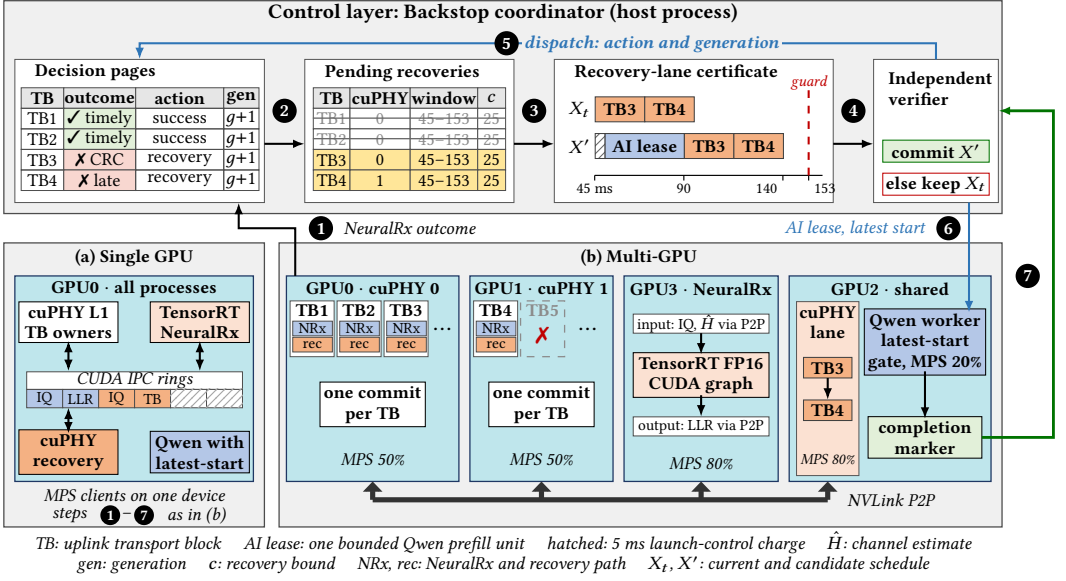
Fig. 5. Backstop architecture for one release period. Steps: NeuralRx outcome (①), outcome batch (②), recovery retiming (③), independent verification (④), dispatch (⑤), AI lease (⑥), and completion marker (⑦). The steps are drawn for the evaluated multi-GPU placement (b); the single-GPU placement (a) exchanges IQ, LLR, and TB buffers through CUDA IPC rings and uses the same steps. In (b), cuPHY instance 0 owns TB1-TB3, instance 1 owns TB4 and TB5, and ellipses mark further TBs.
