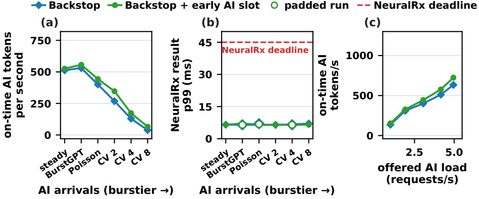
Fig. 16. Early AI slots on one GPU, paired with Backstop without them. (a) On-time AI tokens per second under the six arrival patterns at 3 requests/s. (b) p99 of the NeuralRx release-to-result path in natural runs (lines) and padded runs (circles), against the 45 ms NeuralRx deadline. (c) On-time AI tokens per second against the offered Poisson load, with a 200 ms AI SLO.
