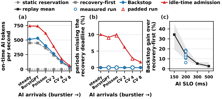
Fig. 13. AI service and radio safety under bursty AI arrivals on the physical multi-GPU path. Every pattern carries the same 329 BurstGPT prompts at 3 requests/s for 108 s and differs only in arrival times; the AI SLO is 200 ms. (a) AI tokens served within their SLO; static reservation admits no AI request. (b) Periods in which the admitted AI misses the recovery deadline at the declared bounds (lines, measured service times), and periods whose last recovery physically ends after the recovery deadline when every AI request and recovery takes its bound (padded runs). (c) Gain of Backstop over recovery-first against the AI SLO: replay mean over the six patterns with its range (band), and the measured runs at 200 ms.
