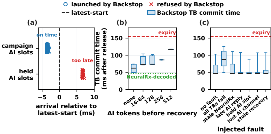
Fig. 18. Schedule enforcement and radio commit time. (a) Arrival of each AI slot at the Qwen worker relative to its absolute latest-start: the 1,077 slots of the two-node campaign and the 52 slots that the held-slot fault keeps past the latest-start. (b) Commit time of every recovered TB in the two-node campaign, grouped by the prompt length of the AI slot that runs before its recovery; the dotted line marks the median commit of the TBs that NeuralRx decodes. (c) Commit time of every TB under each injected fault: no fault, all TBs of a period fail, stale and duplicate NeuralRx outcomes, a late AI reply after GPU completion, an AI slot held past its latest-start, an AI channel lost before GPU completion, and stale and duplicate recovery responses.
