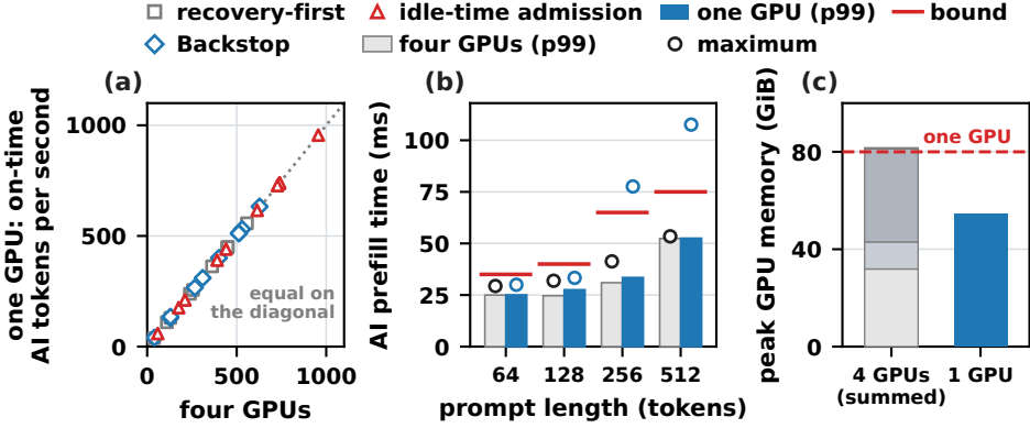
Fig. 15. Single-GPU placement against the paired multi-GPU runs. (a) On-time AI tokens per second of the 30 paired natural runs (six arrival patterns at 3 requests/s and four Poisson loads); the diagonal marks equal service. (b) AI prefill time per prompt length over every run, stopped and padded runs included: p99 (bars) and maximum (circles) against the class bound (red). (c) Peak GPU memory of the multi-GPU placement summed over its four GPUs and of the single-GPU placement with one shared recovery receiver; the dashed line marks the memory of one A100.
