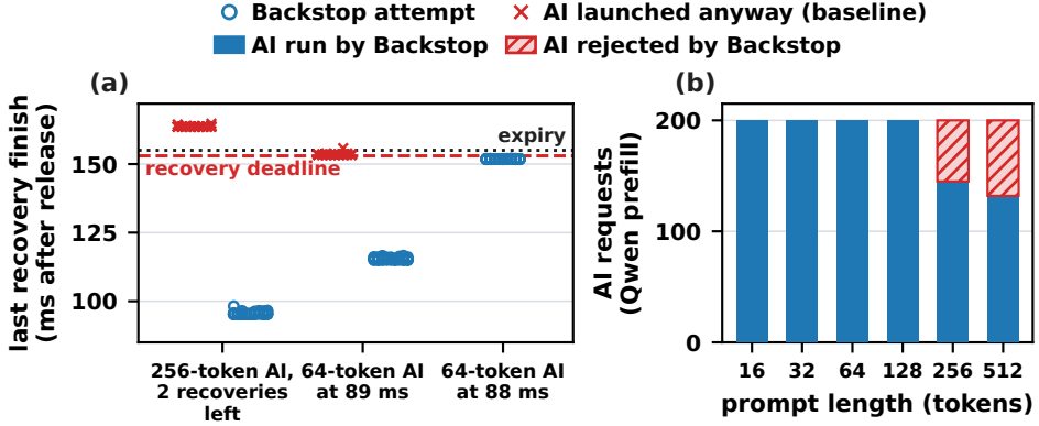
Fig. 17. Radio safety at the admission boundary on two nodes. (a) End of the last recovery in every attempt of the bound-padded boundary diagnostic. E4 offers a 256-token request with two required recoveries at 45 ms; E6b and E6a offer a 64-token request with one required recovery at 89 and 88 ms. Baseline attempts launch the request anyway: idle-time admission in E4 and a forced launch of the request that Backstop rejects in E6b. (b) AI requests per prompt length in the two-node campaign: requests that Backstop runs and requests that it rejects because the required recoveries would then miss the recovery deadline; idle-time admission would run all of them, and static reservation runs none.
