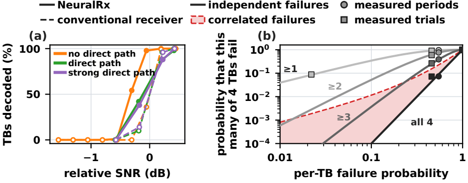
Fig. 2. Uncertain recovery need across channels and failure rates. (a) Share of TBs that NeuralRx (solid) and the conventional receiver (dashed) decode in three channels: a synthetic fading channel without a direct path (block Rayleigh) and two 3GPP channels with a direct path (CDL-D) and a strong direct path (CDL-E); the relative SNR is 0 dB where the conventional receiver decodes half of the TBs. (b) Probability that one or more, two or more, three or more, or all four TBs of a period fail when each TB fails with probability p . Lines assume independent failures; the band raises the correlation of the all-four event to 0.3. Circles are measured periods that join the transition-SNR TBs of two consecutive campaign periods; squares are grouped trials of four consecutive receiver trials.
