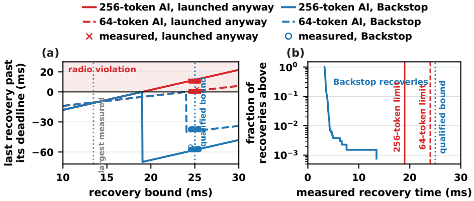
Fig. 20. Sensitivity to the recovery bound. (a) End of the last recovery relative to the recovery deadline when the request that Backstop rejects runs anyway, against the recovery bound B_{\text{conv}} : lines follow the bound-respecting schedules of the 256-token case (E4) and the 64-token case (E6b), and markers show the physical attempts measured at the qualified 25 ms bound. (b) Share of the 1,312 measured recovery times of the two-node campaign that exceed a given length, with the bounds at which each case disappears (limits) and the qualified bound.
