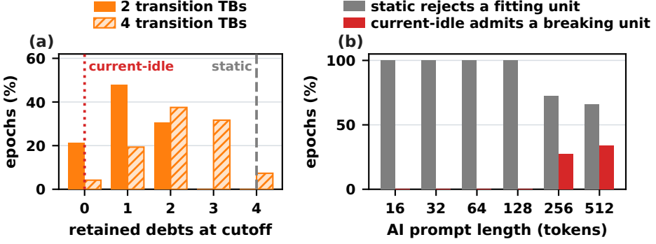
Fig. 2. Measured recovery debt in the evaluated warm mode (1,200 epochs on two nodes). (a) Retained debts at the 45 ms common cutoff for epochs with two transition-SNR TBs, and for 600 four-TB epochs that join the transition TBs of consecutive measured epochs. The dotted line marks the zero debt that current-idle admission sees; the dashed line marks the four recoveries that static reservation holds. (b) Share of epochs, per AI prompt length, in which static reservation rejects a unit that the all-fail certificate admits and in which current-idle admission accepts a unit that breaks the all-fail recovery bound.
