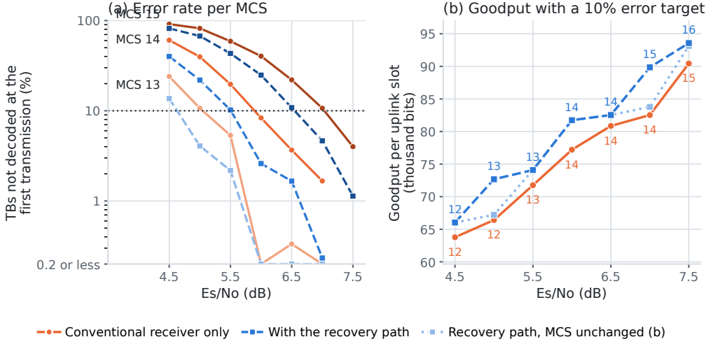
Fig. 12. Link adaptation with the recovery path (two-user cell, low-correlation channel, 300 TBs per point). Dotted line in (a): 10% target. Numbers in (b): MCS chosen.
