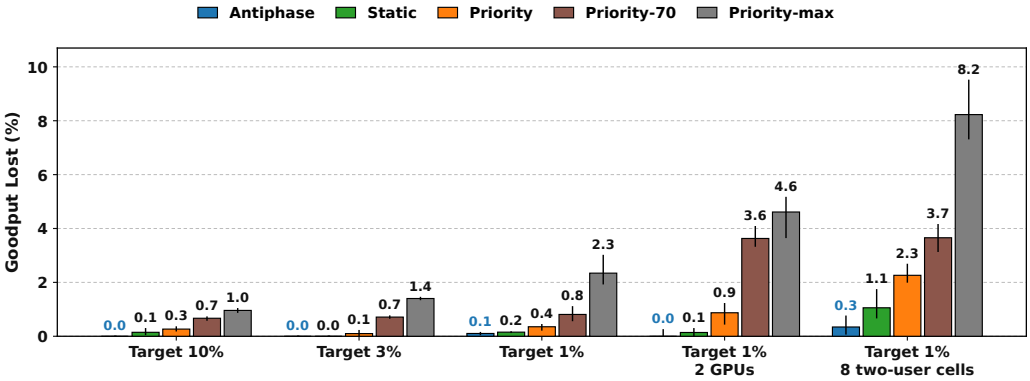
Fig. 13. Goodput of the two-user cells that each policy loses against the same server without AI, with an outer-loop rate controller (target: share of TBs that need a retransmission; lines show the range over seeds).
