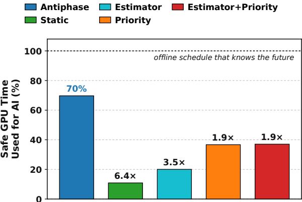
Fig. 10. Share of the GPU time that is safe for AI that each policy turns into served tokens at a steady full load (16 cells, four GPUs). 100% is an offline schedule that knows every later failure and loses no recovery. The number on a baseline is the factor of Antiphase over it.
