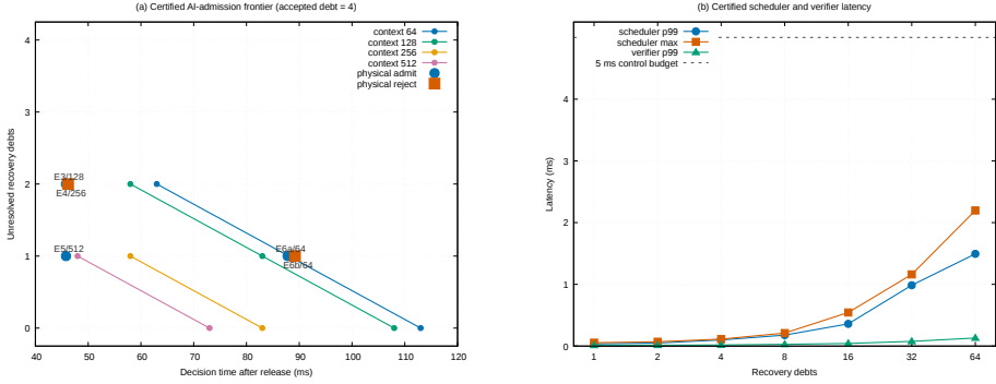
Fig. 10. Predictive scheduling and control cost. (a) The qualified AI-admission frontier moves with recovery debt, AI class, and decision time; prespecified physical cases lie on the predicted side. (b) Candidate construction and independent verification remain below the evaluated 5 ms control budget through 64 debts. Latencies are finite-run measurements, not WCETs.
