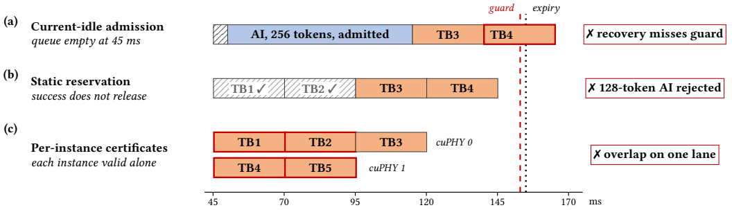
Fig. 4. Scheduling failures after two timely successes (TB1, TB2). (a) Current-idle admission pushes a retained recovery past the guard. (b) Static reservation rejects a 128-token AI unit that fits once the successful reservations are released. (c) Per-instance certificates claim one lane interval.
