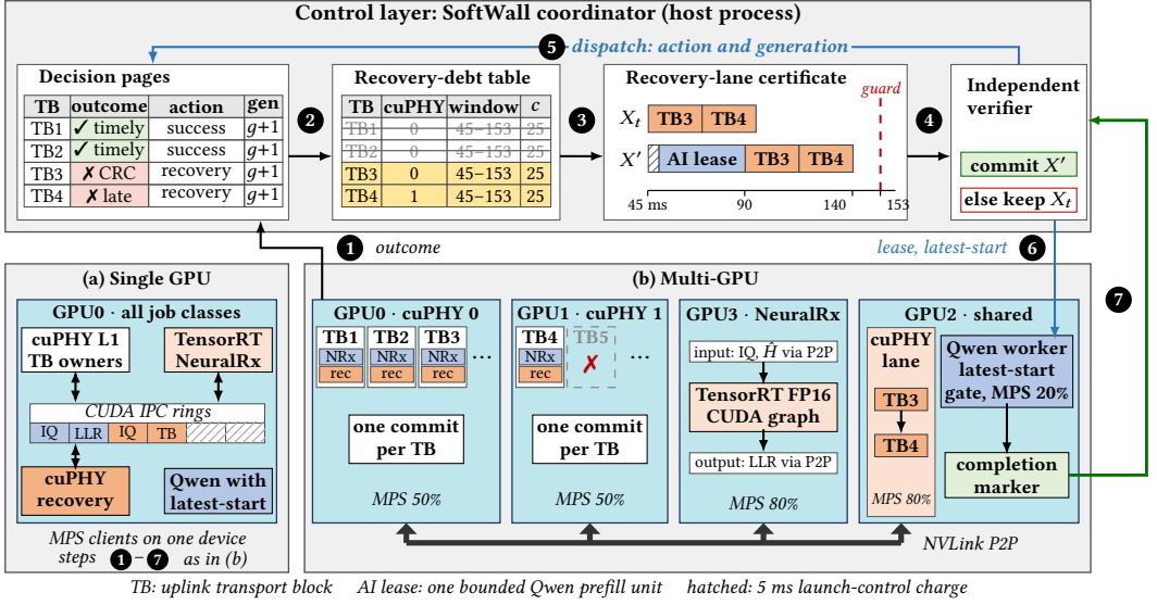
Fig. 5. SoftWall architecture for one epoch. (1) Each owner publishes its NeuralRx outcome to a decision page. (2) One common-cutoff batch updates the recovery-debt table. (3) The scheduler retimes retained debts around a candidate AI lease. (4) The independent verifier checks the all-fail schedule, credits, and generation, and commits X' or keeps X_t . (5) The coordinator publishes each action with its generation and (6) sends the lease with an absolute latest-start. (7) A completion or non-launch marker retires the lease. The shared lane runs retained recoveries in certificate order. The steps are drawn for the evaluated multi-GPU placement (b); the single-GPU placement (a) exchanges IQ, LLR, and TB buffers through CUDA IPC rings and uses the same steps. In (b), cuPHY instance 0 owns TB1–TB3, instance 1 owns TB4 and TB5, and ellipses mark further TBs.
