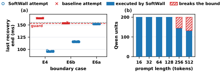
Fig. 11. Radio safety and AI admission under physical execution on two nodes. (a) End of the last recovery in every attempt of the bound-padded boundary diagnostic; baseline attempts are idle-time admission in E4 and the shadow launch of the unit that SoftWall rejects in E6b. (b) Qwen units per prompt length in the two-node campaign: units executed by SoftWall and units that only idle-time admission would launch because they break the certified recovery bound; static reservation launches none.
