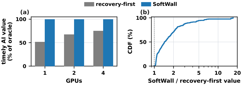
Fig. 10. Timely AI value on BurstGPT traces at the 362 prespecified headroom points. (a) Mean timely value relative to the fixed-placement oracle per GPU count. (b) CDF of the ratio between the timely value of SoftWall and that of certificate-preserving recovery-first.
