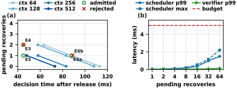
Fig. 12. Predictive scheduling and control cost. (a) Latest decision time at which one AI unit of each prompt length remains admissible with four admitted TBs and zero to four pending recoveries; circles and crosses mark the prespecified physical cases that the scheduler admitted and rejected. (b) Candidate construction and independent verification latency against the number of pending recoveries, with the evaluated 5 ms control budget. Latencies are finite-run measurements, not WCETs.
