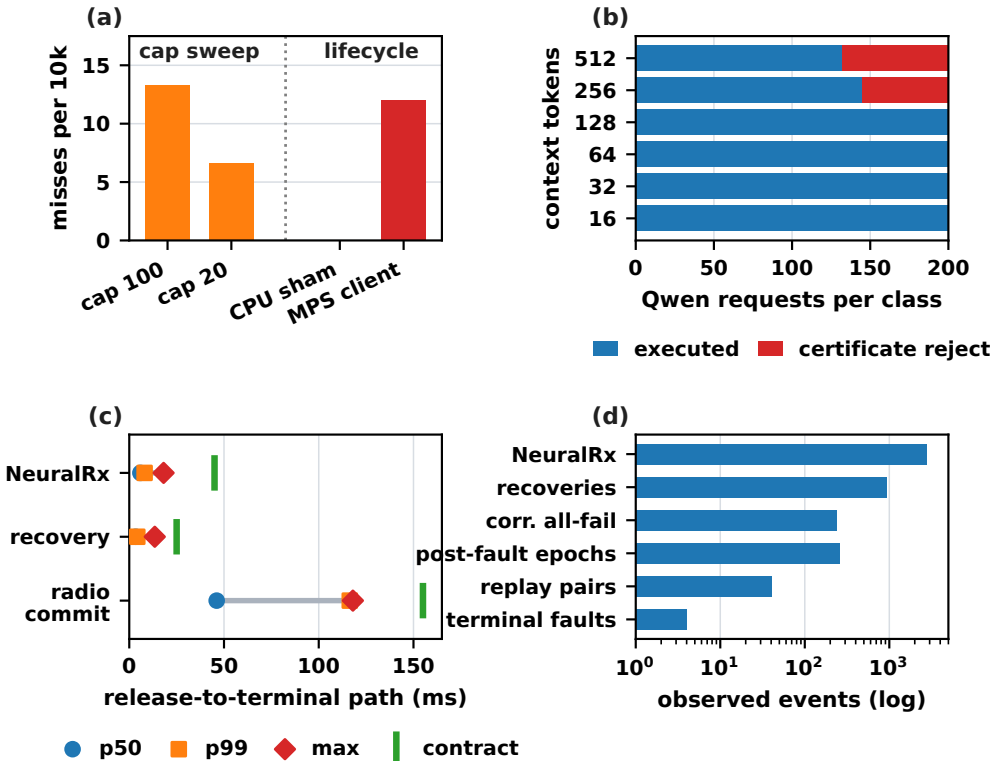
Fig. 10. Physical evidence for the scheduling contract. (a) MPS cap-only and lifecycle diagnostics retain deadline misses. (b) The scheduler admits every offered 16–128-token Qwen unit and rejects larger classes when recovery debt consumes the window. (c) Whole-path samples remain inside their mode contracts. (d) The fault campaign spans frequent execution and rare terminal events without an observed deadline or invariant violation.
