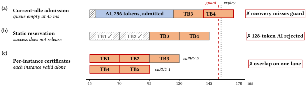
Fig. 3. Scheduling failures after two timely successes (TB1, TB2). (a) Current-idle admission pushes a retained recovery past the guard. (b) Static reservation rejects a 128-token AI unit that fits once the successful reservations are released. (c) Per-instance certificates claim one lane interval.
