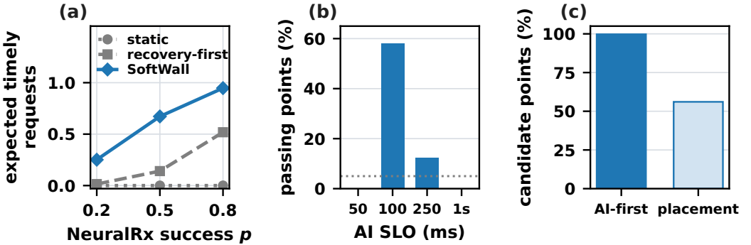
Fig. 8. Scheduling capacity and decision quality. (a) Expected timely requests at a representative four-cell, two-instance, one-GPU point with correlated outcomes. (b) Fraction of 513 mandatory-feasible trace points per SLO that pass the frozen 5% headroom screen. (c) Of 362 advanced points, a safe AI-first greedy is within 5% of the fixed-placement oracle at 361; flexible recovery placement has a positive upper-bound gain at 203.
