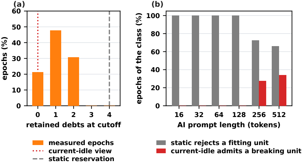
Fig. 2. Measured recovery debt in the evaluated warm mode (1,200 epochs on two nodes). (a) Retained debts at the 45 ms common cutoff; the dotted line marks the zero debt that current-idle admission sees, and the dashed line marks the four recoveries that static reservation holds. (b) Share of epochs, per AI prompt length, in which static reservation rejects a unit that the all-fail certificate admits and in which current-idle admission accepts a unit that breaks the all-fail recovery bound.
