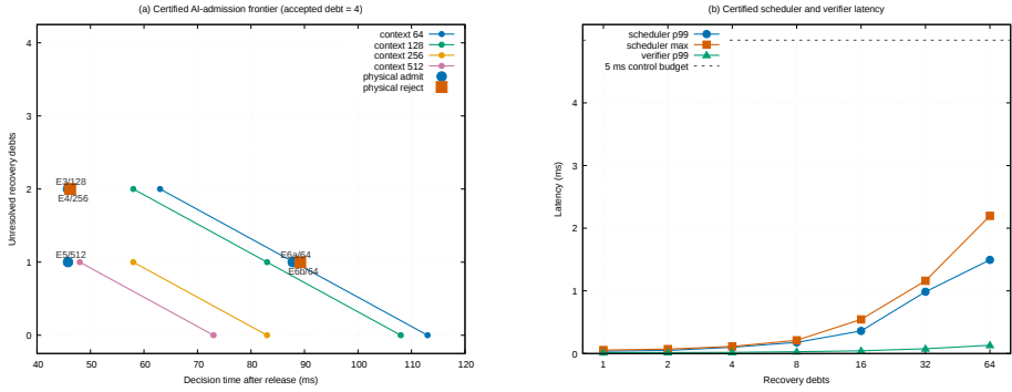
Fig. 9. Predictive scheduling and control cost. (a) The qualified AI-admission frontier moves with recovery debt, AI class, and decision time; prespecified physical cases lie on the predicted side. (b) Candidate construction and independent verification remain below the evaluated 5 ms control budget through 64 debts. Latencies are finite-run measurements, not WCETs.
