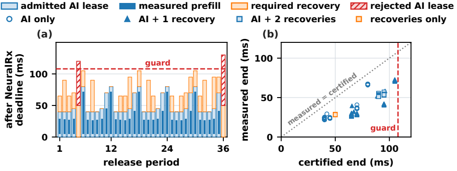
Fig. 11. Online scheduling in the two-node campaign, measured from the NeuralRx deadline. (a) Certificate of the shared lane in 36 consecutive release periods: each admitted AI lease includes the 5 ms launch-control charge, and the required recoveries follow it with their full bound; a rejected AI lease is drawn where it would end. (b) Measured against certified end of the last lane action in all 1,200 periods; the dotted diagonal marks equality.
