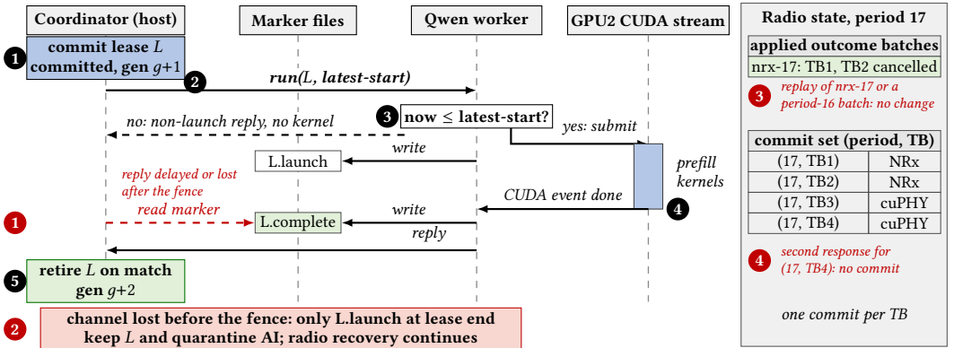
Fig. 7. Refinement of one AI lease. Black steps: commit with a latest-start (❶), run request (❷), launch gate and launch marker (❸), CUDA event and completion marker (❹), and retirement on a matching marker (❺). Red faults: marker reconciliation after a late reply (❶), AI quarantine after channel loss (❷), and no-op outcome and response replays (❸, ❹).
