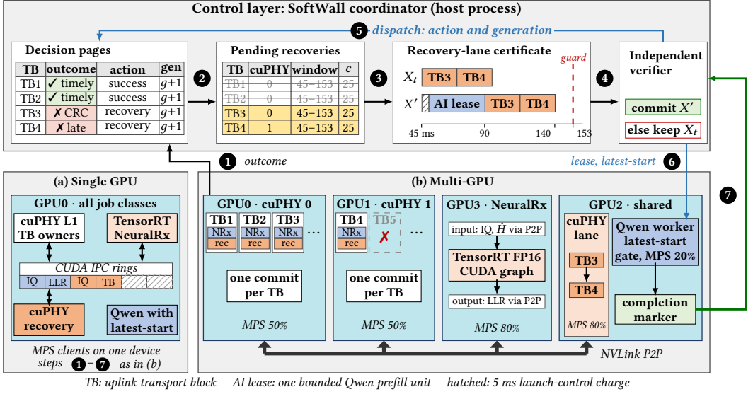
Fig. 5. SoftWall architecture for one release period. Steps: NeuralRx outcome (①), outcome batch (②), recovery retiming (③), independent verification (④), dispatch (⑤), AI lease (⑥), and completion marker (⑦). The steps are drawn for the evaluated multi-GPU placement (b); the single-GPU placement (a) exchanges IQ, LLR, and TB buffers through CUDA IPC rings and uses the same steps. In (b), cuPHY instance 0 owns TB1-TB3, instance 1 owns TB4 and TB5, and ellipses mark further TBs.
