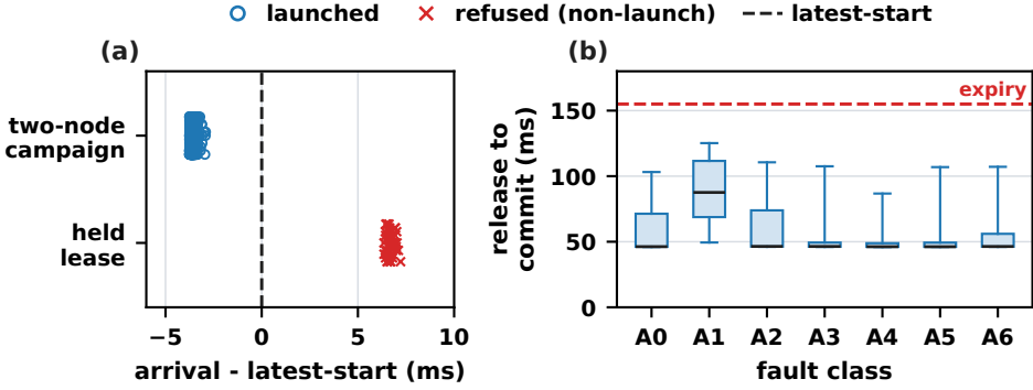
Fig. 13. Execution refinement under physical faults. (a) Arrival of each AI lease at the Qwen worker relative to its absolute latest-start: the 1,077 leases of the two-node campaign and the 52 leases that fault class A4 holds past the latest-start. (b) Release-to-commit time of every TB in fault classes A0-A6: no fault, correlated all-fail, stale and duplicate NeuralRx outcomes, Qwen reply delay after the fence, lease held past the latest-start, Qwen channel loss before the fence, and stale and duplicate recovery responses.
