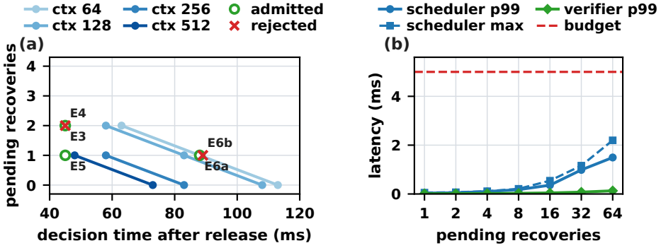
Fig. 14. Predictive scheduling and control cost. (a) Latest decision time at which one AI unit of each prompt length remains admissible with four admitted TBs and zero to four pending recoveries; circles and crosses mark the prespecified physical cases that the scheduler admitted and rejected. (b) Candidate construction and independent verification latency against the number of pending recoveries, with the evaluated 5 ms control budget. Latencies are finite-run measurements, not WCETs.
