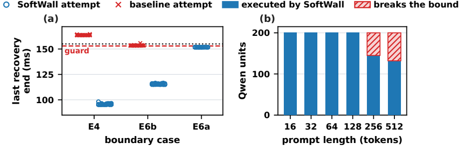
Fig. 12. Radio safety at the certificate boundary on two nodes. (a) End of the last recovery in every attempt of the bound-padded boundary diagnostic; baseline attempts are idle-time admission in E4 and the shadow launch of the unit that SoftWall rejects in E6b. (b) Qwen units per prompt length in the two-node campaign: units executed by SoftWall and units that only idle-time admission would launch because they break the certified recovery bound; static reservation launches none.
