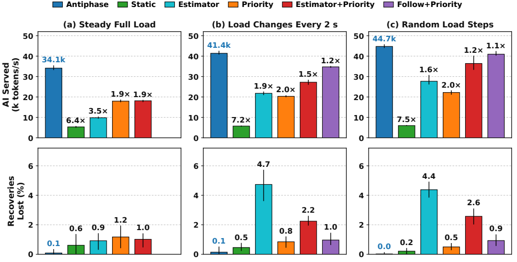
Fig. 6. AI served (top) and recoveries lost (bottom) under three load patterns (16 cells, four GPUs, five seeds; lines show the range over seeds). The number on a baseline is how many times more AI Antiphase serves than that baseline.
