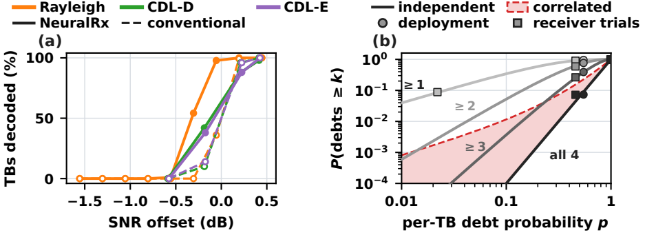
Fig. 3. Uncertain recovery debt across channels and failure rates. (a) Share of TBs that NeuralRx (solid) and the conventional receiver (dashed) decode in three channel models; each SNR is shifted so that the conventional receiver decodes half of the TBs at 0 dB. (b) Probability that an epoch with four admitted TBs retains at least k debts when each TB fails with probability p . Lines assume independent failures; the band raises the correlation of the all-four event to 0.3. Circles are deployment epochs that join the transition-SNR TBs of two consecutive measured epochs; squares group four consecutive receiver trials.
