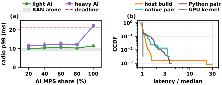
Fig. 2. Execution variability on shared A100 GPUs. (a) Radio p99 of a two-cell 273-PRB PUSCH pipeline against the MPS share of a co-running Qwen prefill class: one 16-token request (light) or eight 512-token requests (heavy). Lines connect run means, and bars span the runs. (b) Complementary CDF of latency normalized by its median: host construction of a scheduling certificate (1,200 epochs), cross-GPU receiver pairs at the 4.5 ms scale with a Python and a partly native C++/CUDA path (1,000 and 300 slots), and the NeuralRx TensorRT graph (300 slots).
