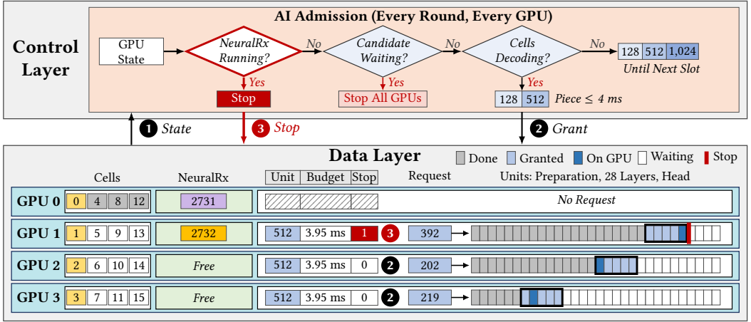
Fig. 4. AI admission with the values of a measured run at the instant the neural receiver of GPU 1 starts the TB of slot 2732 (Figure 2). Top: the decision of AI Admission for one GPU. Bottom: the cells (gray: decoding), the neural receiver, the grant, and the 30 units of the AI request of every GPU. Numbers mark the steps of the text.
