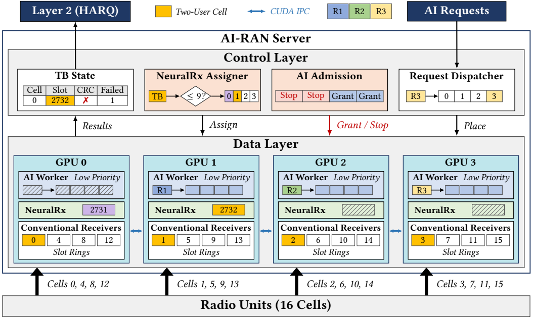
Fig. 1. Overall architecture of Antiphase. Every GPU runs the conventional receivers of four cells, one neural receiver, and one AI worker. The contents of the boxes show the instant of Figures 2 and 4: two neural receivers are busy, and the AI workers of GPU 1-3 hold a request.
