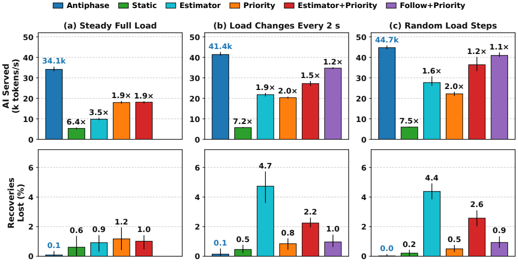
Fig. 6. AI served (top) and recoveries lost (bottom) under three load patterns (16 cells, four GPUs, five seeds; lines show the range over seeds). The number on a baseline is how many times more AI Antiphase serves than that baseline.
