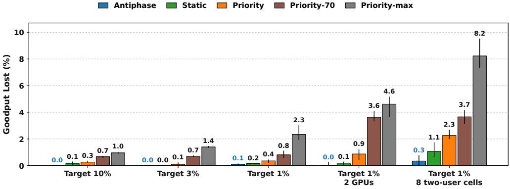
Fig. 11. Goodput of the two-user cells that each policy loses against the same server without AI, with an outer-loop rate controller (target: share of TBs that need a retransmission; lines show the range over seeds).
