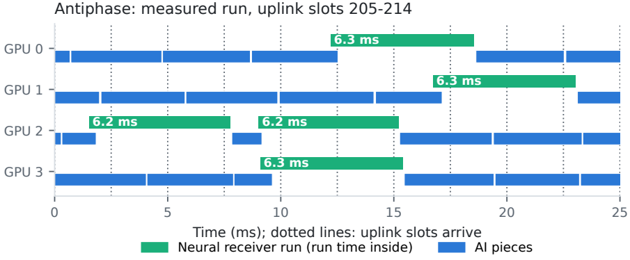
Fig. 5. Measured timeline of the four GPUs under Antiphase (16 cells, full load, 25 ms).
