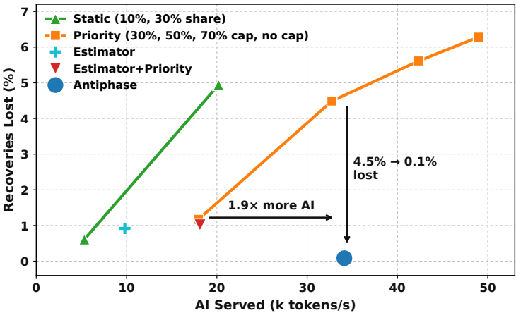
Fig. 9. AI served against recoveries lost at a steady full load (16 cells, four GPUs). A baseline that takes a larger share moves up along its line.
