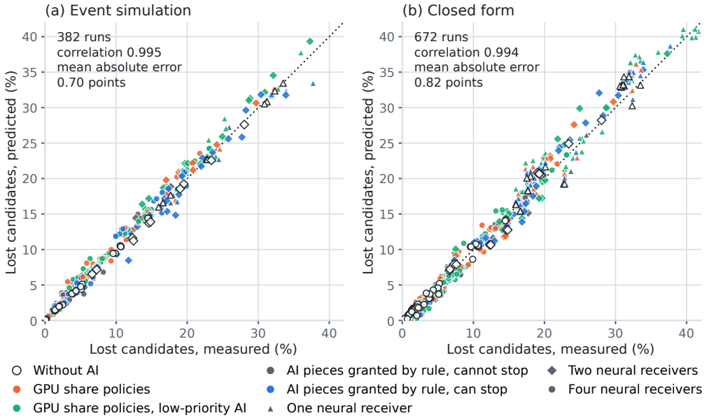
Fig. 7. Share of the candidates that find no free neural receiver, predicted against measured, for every run. GPU share policies: fixed share, share that follows the load, and share chosen by an estimator.
