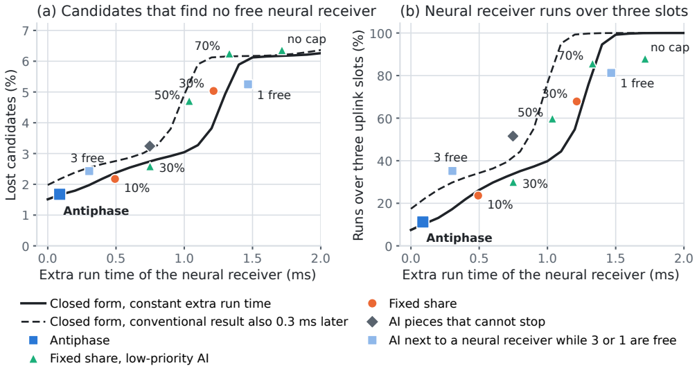
Fig. 8. Lost candidates and three-slot runs against the extra run time of the neural receiver (16 cells, four neural receivers). Lines: closed form with the arrivals and run lengths of the run without AI plus a constant extra run time. Points: measured policies at their median extra run time; labels give the MPS shares.
