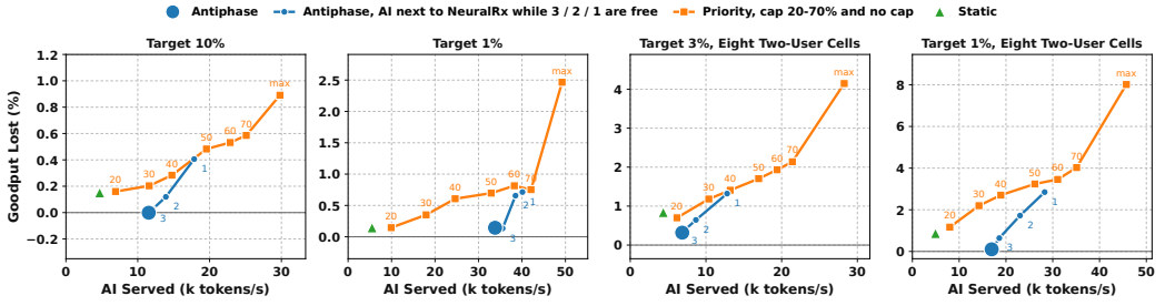
Fig. 12. AI served against the goodput of the two-user cells that is lost, with the outer loop (three seeds; all policies of a panel run in one job). Orange: low-priority AI with a cap of 20-70% and without a cap. Blue: Antiphase, and its settings that allow AI next to a neural receiver while 3, 2, or 1 neural receivers are free.
