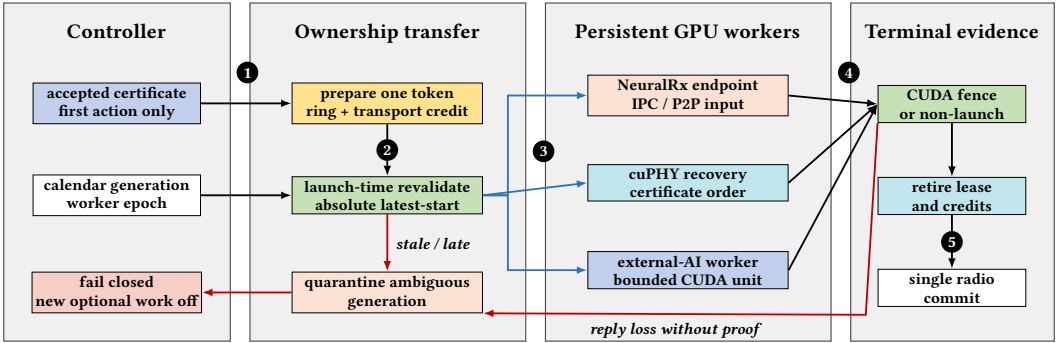
Fig. 5. Certificate-to-execution refinement. (1) A certificate authorizes only its first non-preemptive action. (2) Prepare owns one generation-tagged token. (3) The worker revalidates an absolute latest-start before launch. (4) Persistent NeuralRx, cuPHY, or AI workers publish physical completion. (5) Only matching CUDA fences or qualified non-launch markers retire ownership; stale or ambiguous effects are quarantined.
