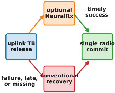
Fig. 1. AI-RAN scheduling background. (a) A timely NeuralRx result may commit directly, but failure, lateness, or missing evidence makes conventional recovery mandatory for the same TB. (b) Multiple RAN homes use local NeuralRx endpoints while their recovery and external-AI work contend on a shared GPU lane through CUDA IPC or NVLink P2P.
