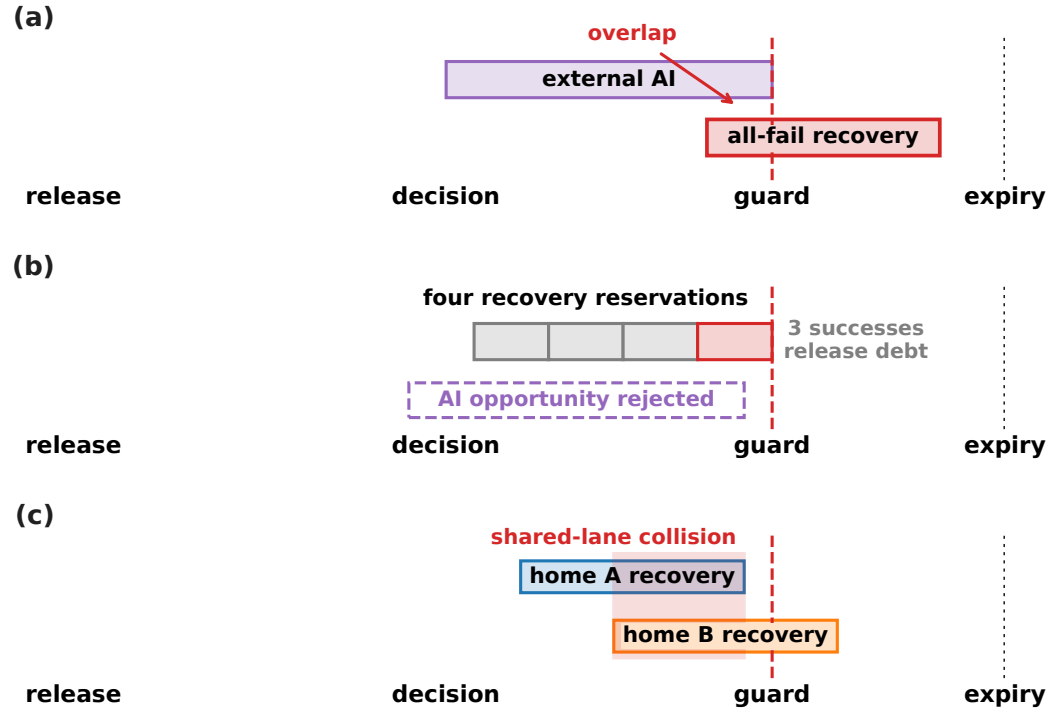
Fig. 2. Why existing scheduling abstractions are insufficient. (a) Current-idle admission can overlap a future all-fail recovery. (b) Static reservation is safe but rejects an AI opportunity that timely NeuralRx successes could release. (c) Per-home certificates can overlap after composition on the shared cuPHY lane. Dashed vertical lines mark the radio guard and expiry.
