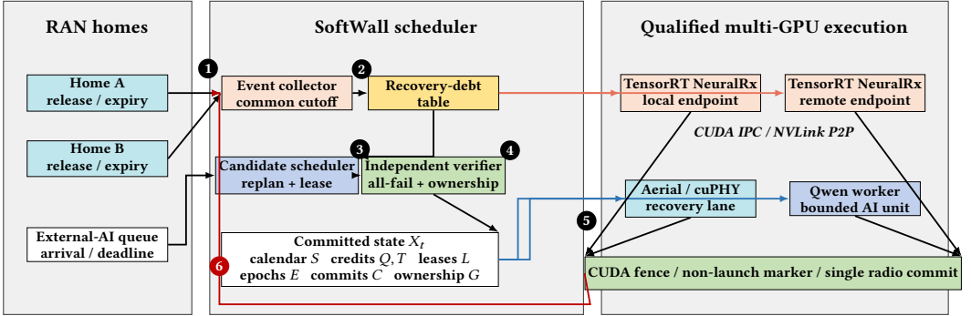
Fig. 3. Overall SoftWall architecture. (1) Homes and AI queues publish only currently visible events. (2) Each unresolved optional receiver owns conventional-recovery debt. (3) The candidate scheduler jointly retimes debt and proposes an AI lease. (4) An independent verifier checks the complete state. (5) Only a verified state grants dispatch authority. (6) Receiver outcomes and terminal fences trigger the next atomic transition.
