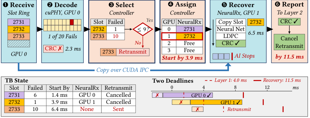
Fig. 2. Recovery path as six steps, with three consecutive failed TBs of one cell in a measured run (cell 0, slots 2731-2733). Blue steps run on a GPU and peach steps in the controller. Every TB keeps its color. Bottom: TB State after the six steps and the two deadlines of every TB; times count from the arrival of the samples of slot 2732.
