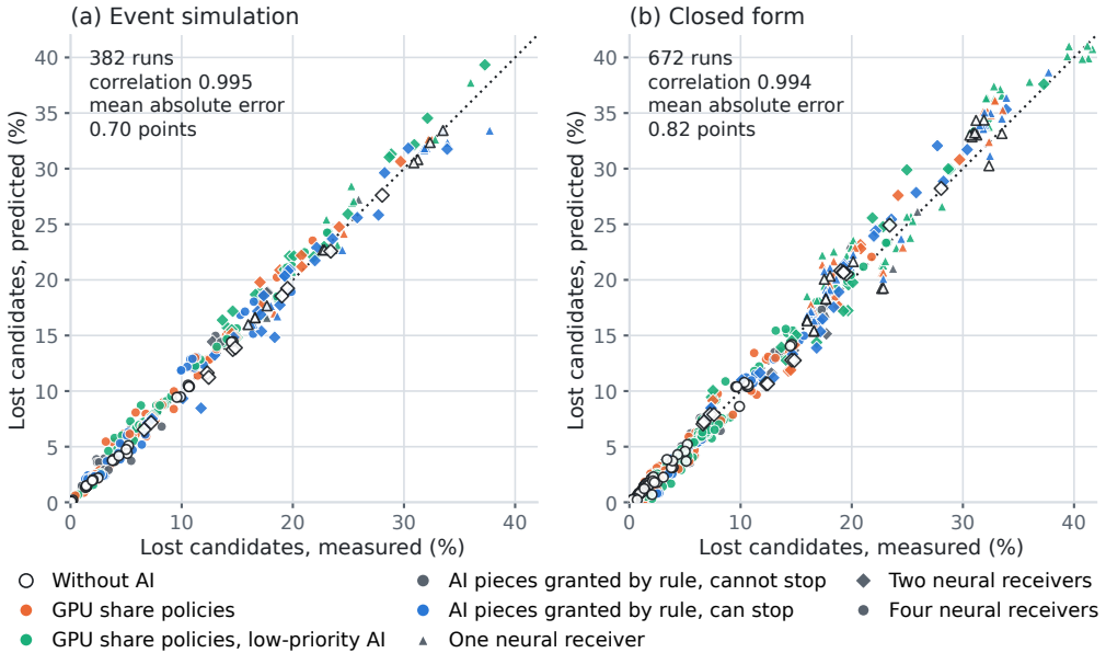
Fig. 7. Share of the candidates that find no free neural receiver, predicted against measured, for every run. GPU share policies: fixed share, share that follows the load, and share chosen by an estimator.
