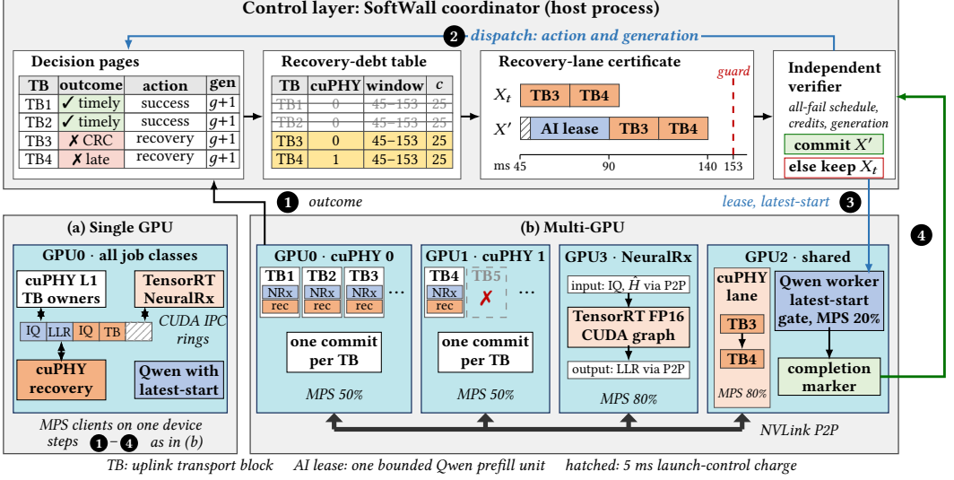
Fig. 3. SoftWall architecture. The numbered steps are drawn for the evaluated placement (b); the single-GPU placement (a) uses the same decision pages, lease RPC, and markers. (1) Each owner publishes its NeuralRx outcome to a decision page. One common-cutoff batch then updates the debt table, the scheduler retimes retained debts around a candidate lease, and the independent verifier commits X' or keeps X_t . (2) The coordinator publishes each action with its generation and (3) sends the lease with an absolute latest-start through the AI lease RPC. (4) A completion or non-launch marker retires the lease. The shared lane runs retained recoveries in certificate order. In (a), the processes on one GPU exchange IQ, LLR, and TB buffers through CUDA IPC rings. In (b), the evaluated multi-GPU placement uses NVLink P2P; cuPHY instance 0 owns TB1–TB3, instance 1 owns TB4 and TB5, and ellipses mark further TBs.
