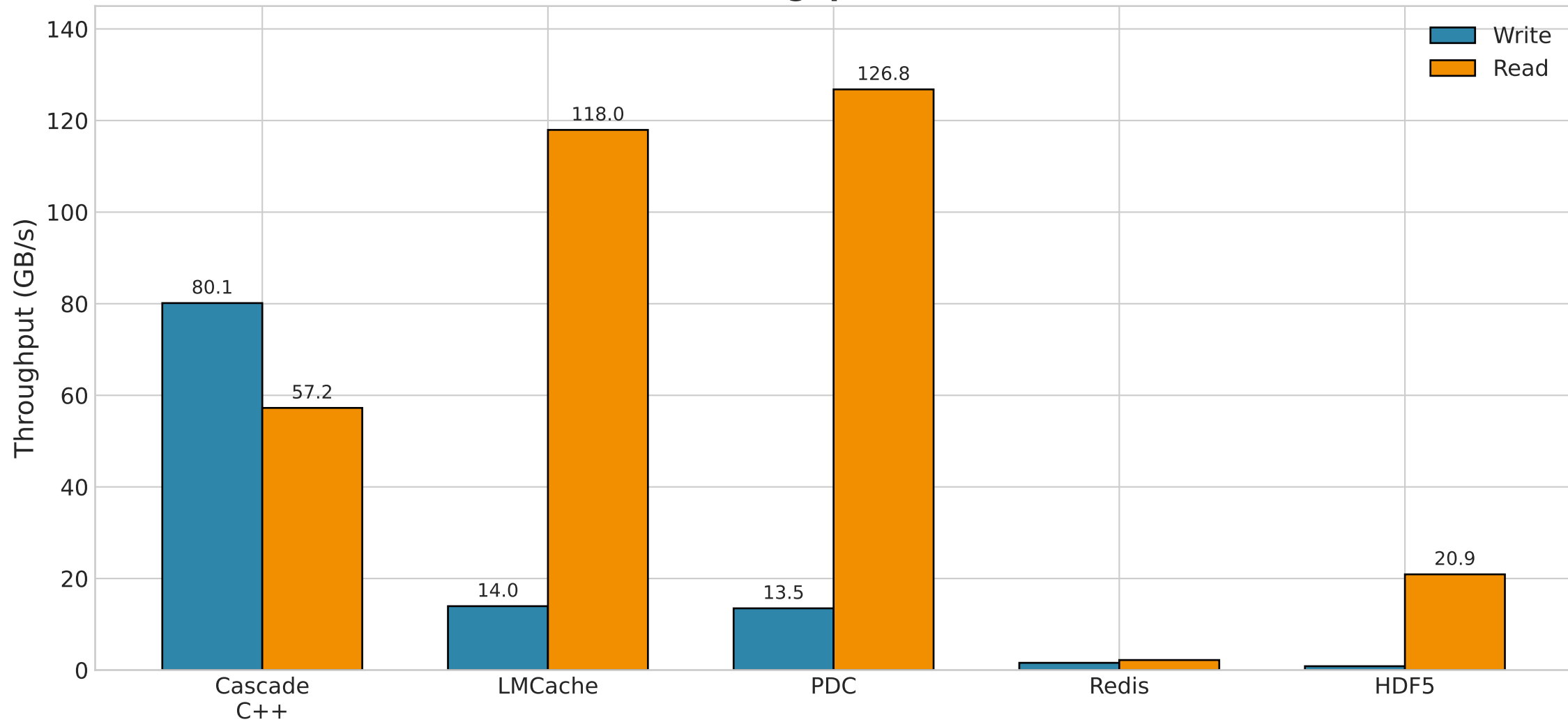
Write vs Read Throughput (16 ranks, 4 nodes)
