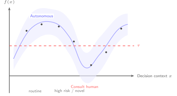
Figure 8: Conceptual illustration of the Trust GP. The blue curve shows the posterior mean of f(x) ; the shaded band shows posterior uncertainty. The dashed threshold \tau defines the HITL boundary: the system operates autonomously when f(x) > \tau and consults a human otherwise. Dots represent observed preference pairs. High-uncertainty regions (e.g., novel contexts around x \approx 3.5 ) fall below the threshold even if the mean is moderate.
