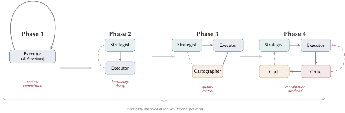
Figure 1: Architectural evolution across four observed phases. Each transition was triggered by a persistent bottleneck (shown in red). Solid arrows indicate primary information flow; dashed arrows indicate feedback.
