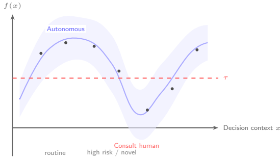
Figure 5: Conceptual illustration of the Trust GP. The blue curve shows the posterior mean of f(x) ; the shaded band shows posterior uncertainty. The dashed threshold \tau defines the HITL boundary: the system operates autonomously when f(x) > \tau and consults a human otherwise. Dots represent observed preference pairs. High-uncertainty regions (e.g., novel contexts around x \approx 3.5 ) fall below the threshold even if the mean is moderate.
