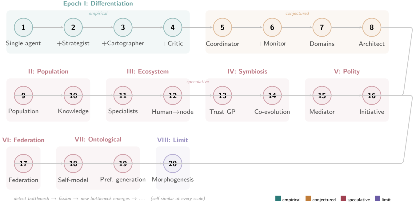
Figure 1: Architectural morphogenesis in an autonomous agent system. A single undifferentiated agent undergoes successive fission events, each triggered by a persistent bottleneck, producing specialized roles. The process mirrors biological cell differentiation: resolving one constraint reliably exposes the next, driving continuous structural change.
