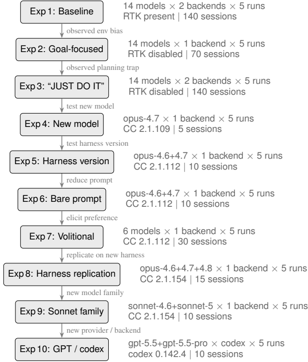
Figure 2. Controlled experiment design. Each experiment was informed by findings from the previous one. Total: 440 sessions across 19 models. CC = Claude Code. Experiment 7 includes 10 primary sessions (opus-4.6/4.7 on Prompt 5) plus 20 supplementary sessions replicating Prompt 3 for the other four Claude models on harness 2.1.112. Experiment 8 replicates the Prompt 5 volitional probe on harness 2.1.154 across opus-4.6/4.7/4.8 (15 sessions).
