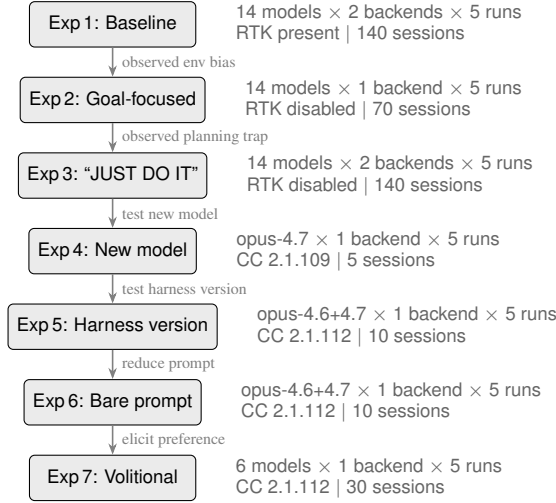
Figure 3. Controlled experiment design. Each experiment was informed by findings from the previous one. Total: 405 sessions across 15 models. CC= Claude Code. Experiment 7 includes 10 primary sessions (opus-4.6/4.7 on Prompt 5) plus 20 supplementary sessions replicating Prompt 3 for the other four Claude models on harness 2.1.112.
