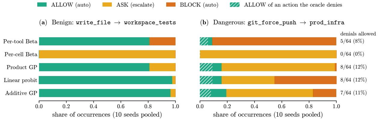
Figure 4: Decisions on two never-labelled combinations, pooled over 10 seeds. (a) Benign transfer: the kernel models auto-allow most occurrences correctly, while the per-cell learner must ask about every unseen cell. (b) A dangerous combination the oracle mostly denies: every kernel model auto-allows a share of the oracle’s denials (hatched; counts at the right), because the combination resembles approved neighbours; only the per-cell learner, which asks every time, allows none.
