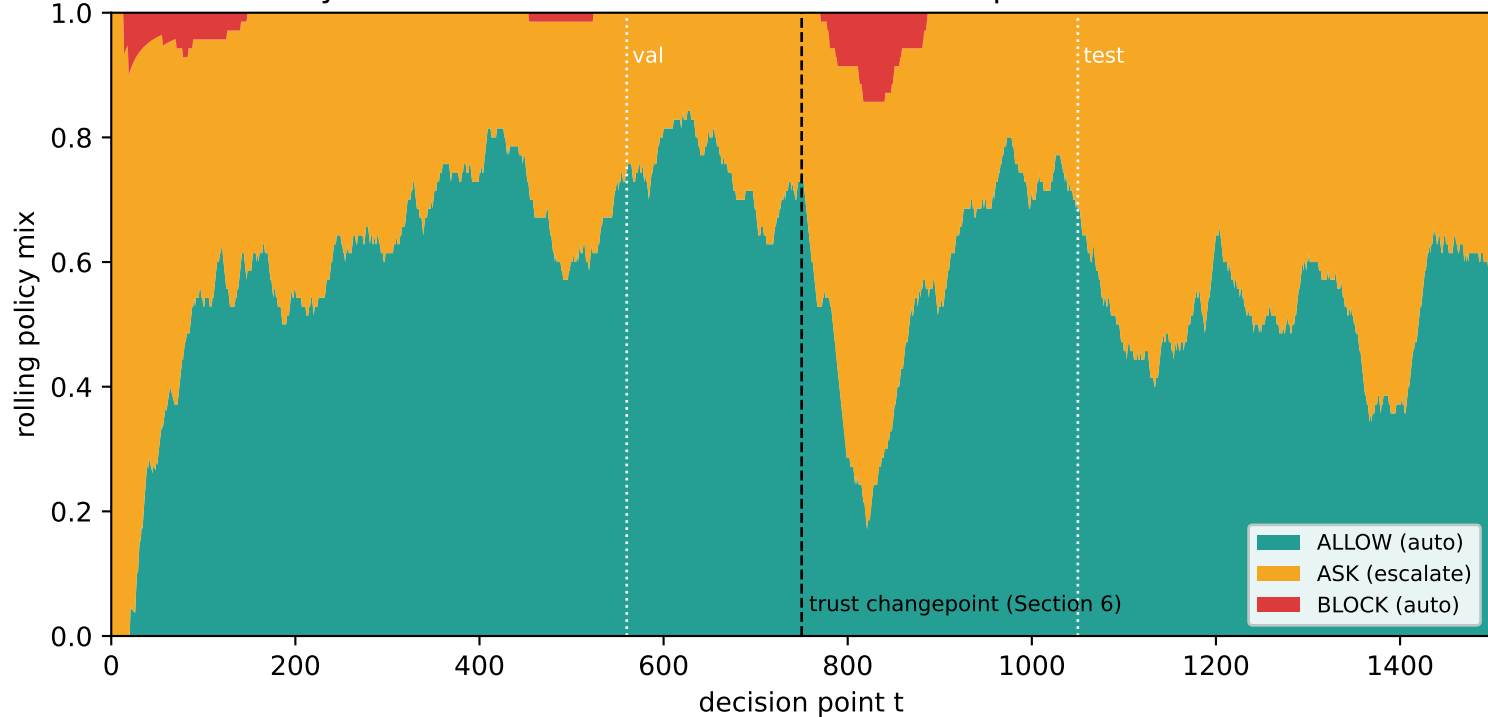
Policy evolution: the ASK band narrows as the posterior concentrates
