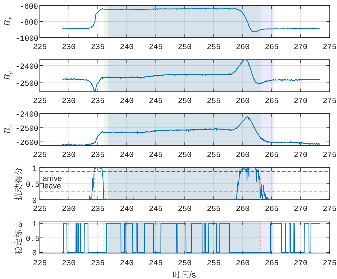
A类波形示例 (GT#4, N_{ev}=1 , stable=0.53, pr=0.132)
